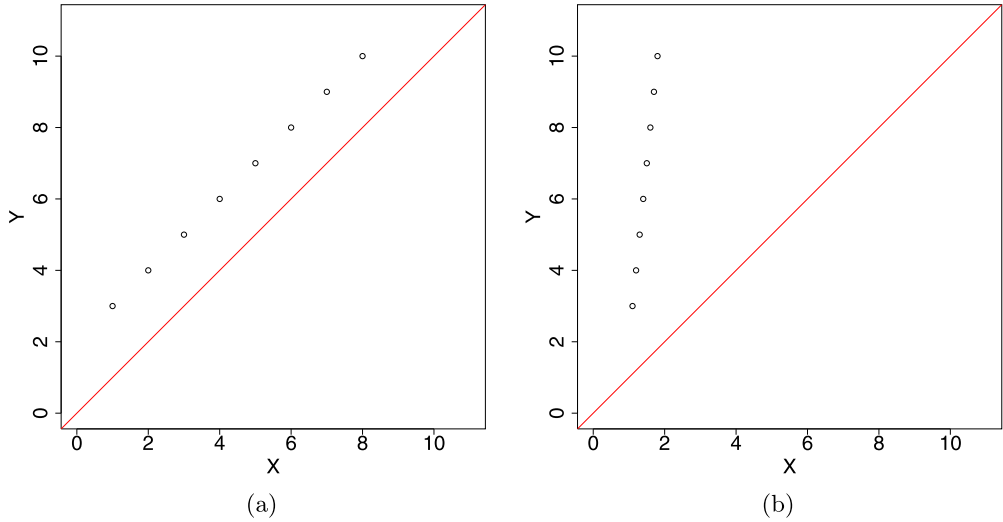
Fig. 1. Departure of two datasets defined on the plane from the 45° line intersecting the origin. (a) Perfect correlation with a shift effect results in relatively high concordance ( \hat{\rho}_c = 0.7241 ). (b) Perfect correlation but poor concordance ( \hat{\rho}_c = 0.0340 ).
