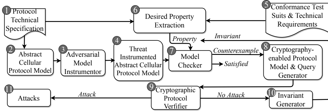
Figure 3: 5GReasoner Architecture.
