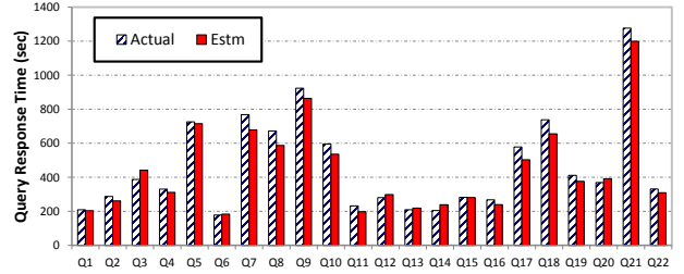
Fig. 7: Accuracy of Query Response Time Prediction
