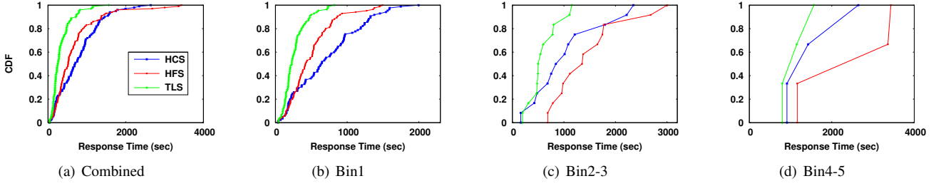
Response Time in Facebook Workload
