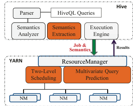
Fig. 4: Semantics-Aware Multivariate Query Modeling and Scheduling
