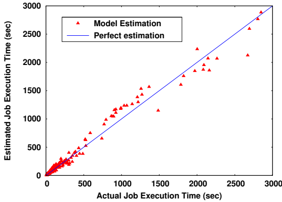
Fig. 6: Accuracy of Job Execution Prediction
