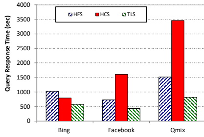
Fig. 14: Average Query Response Times
