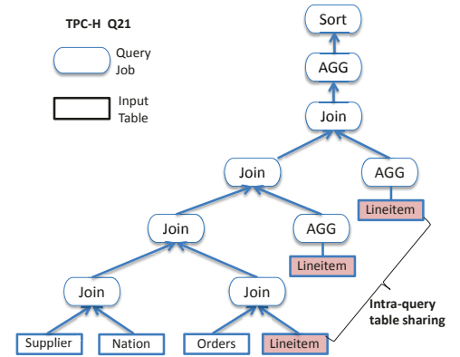
Fig. 10: An Example of Table Sharing for a TPC-H Query
