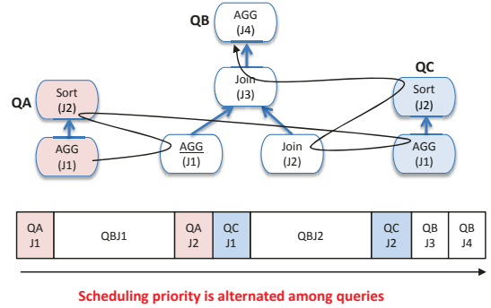
Fig. 1: Under HCS, scheduling priority is alternated among different queries due to semantic unawareness, causing resource thrashing.
