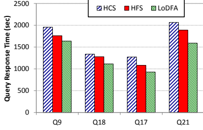
Fig. 11: Query Response Times of Q9, Q18, Q17, and Q21 when They Use System Resources Alone
