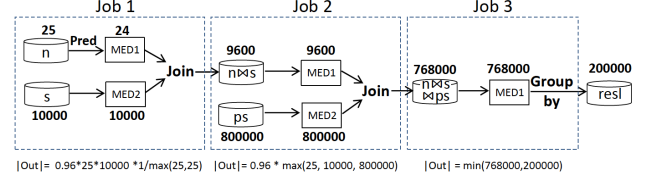
Fig. 5: An Example of Selectivity Estimation
