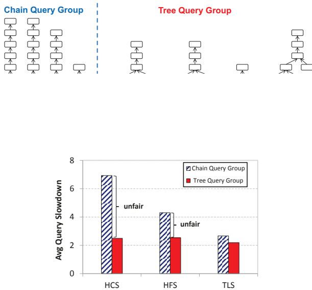
Fig. 3: Fairness to Queries of Different Compositions
