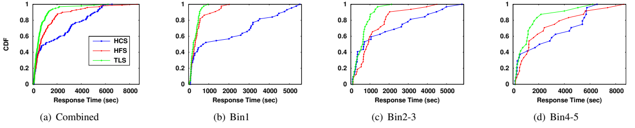
Fig. 15: CDF of Query Response Time in Bing Workload
