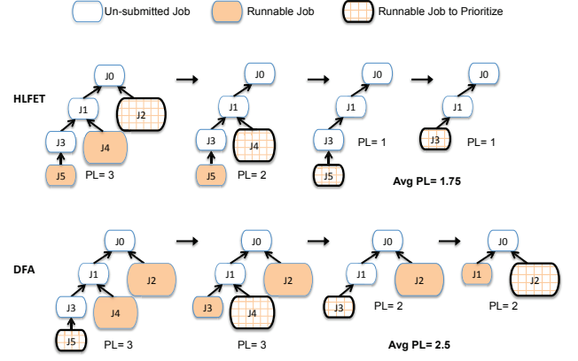
Fig. 9: Comparison between HLFET and DFA Algorithms
