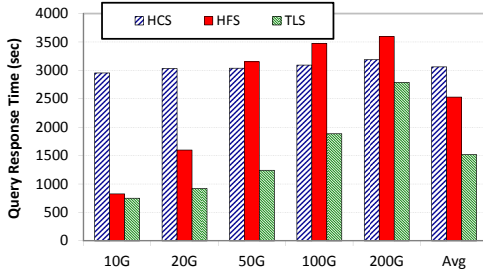
Fig. 17: Query Response Times for Q21 in TPC-H
