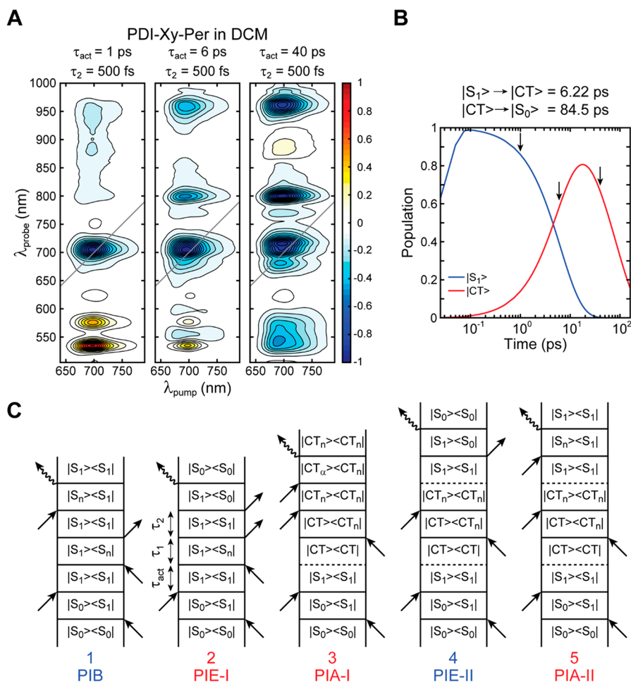
Figure 2. (A) t-2DES spectra of PDI Xy Per in DCM as a function of the actinic pump delay ( \tau_{act} ), where the waiting time ( \tau_2 ) is kept fixed at 500 fs. The spectra are normalized to the maximum absolute change in absorption at each ( \tau_{act} , \tau_2 ). (B) Population evolution of different states obtained from the evolution-associated spectral analysis of conventional 2DES data on PDI-Xy-Per in DCM. The black arrows indicate the actinic delays used for measurement of t-2DES spectra. (C) Feynman diagrams corresponding to representative pathways resulting in different types of t-2DES spectral features. The dotted horizontal lines indicate population transfer during the time period between two light-matter interactions.
