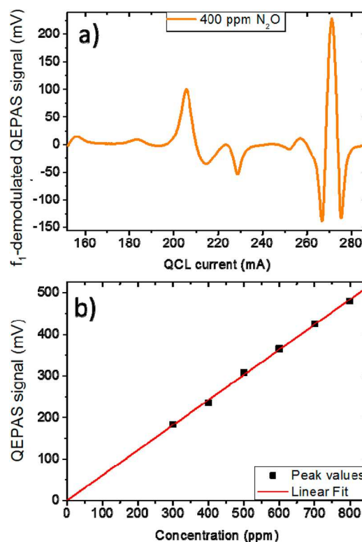
Figure 7. (a) Nitrous oxide spectral scan detected at f_1 exciting the first overtone vibrational mode of the QTF with the quantum cascade laser for a mixture of 400 ppm of nitrous oxide and 1.6% of water in air at 200 Torr. (b) Peak values for each \text{N}_2\text{O} concentration (square symbols) and the corresponding best linear fit (red line).
