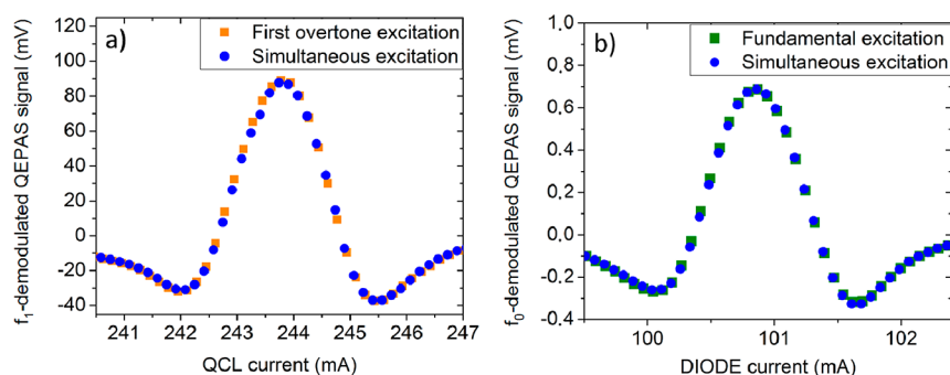
Figure 5. (a) QEPAS spectral scan of the methane absorption line at 1297.47\text{ cm}^{-1} detected at the first overtone mode when only the first overtone mode is excited (orange squares) or both the fundamental and the first overtone modes are excited (blue circles). (b) QEPAS spectral scan of the water vapor absorption line at 7181.16\text{ cm}^{-1} detected at the fundamental mode when only the fundamental mode is excited (green squares) or both the fundamental and first overtone modes are excited (blue circles).
