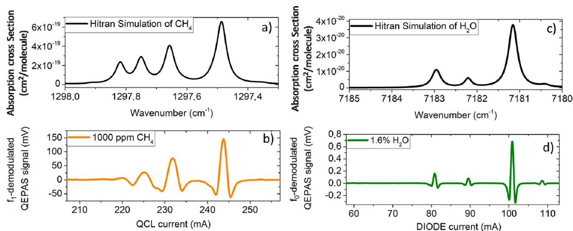
Figure 4. (a) Hitran simulation of the pure methane absorption cross-section at 200 Torr; (b) QEPAS spectral scan of 1000 ppm of CH 4 at 200 Torr measured by demodulating the QTF signal at the overtone mode frequency; (c) Hitran simulation of the pure water vapor absorption cross-section at 200 Torr; (d) QEPAS spectral scan of 1.6% of H 2 O at 200 Torr measured by demodulating the QTF signal at the fundamental mode frequency.
