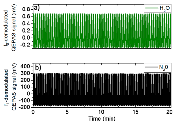
Figure 8. Simultaneous QEPAS spectral scans for a mixture of 600 ppm of nitrous oxide in humidified air. (a) \text{H}_2\text{O} vapor signal detected at f_0 applying a narrow ramp to the diode laser current centered on the water vapor line at 7181.16\text{ cm}^{-1} . (b) \text{N}_2\text{O} signal detected at f_1 applying a narrow ramp to the QCL current centered on the \text{N}_2\text{O} absorption line at 1297.05\text{ cm}^{-1} .
