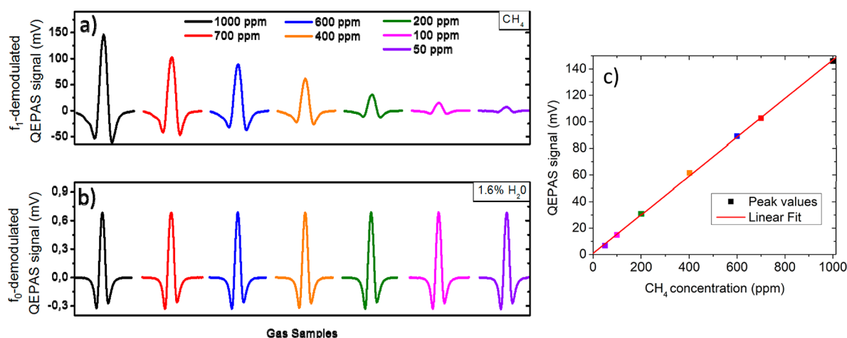
Figure 6. (a) Spectral scans of the methane absorption line at 1297.47\text{ cm}^{-1} for different \text{CH}_4 concentrations in humidified air with 1.6% water vapor. (b) Corresponding spectral scans of the water absorption line at 7181.16\text{ cm}^{-1} for \text{CH}_4 each dilution, confirming that the \text{H}_2\text{O} concentration was kept constant. Simultaneous spectral scans are represented by the same curve color. (c) Peak values for each \text{CH}_4 concentration (square symbols) and the corresponding best linear fit (red line).
