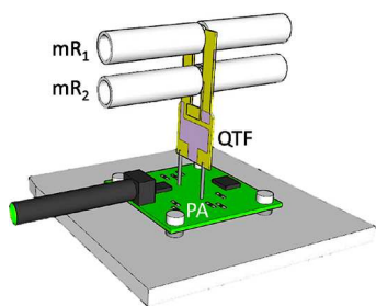
Figure 1. Schematic of the spectrophone implemented. The QTF is coupled with two pairs of microresonator tubes aligned perpendicularly to the QTF. The first pair of tubes ( mR_1 ), each one 9.5 mm long, is located at the fundamental antinode point near the QTF top, the second pair ( mR_2 ), each tube 8.5 mm long, is positioned 9.5 mm below the prongs top, at the second antinode point position of the QTF first overtone mode; the preamplifier (PA) board is shown on the bottom.
