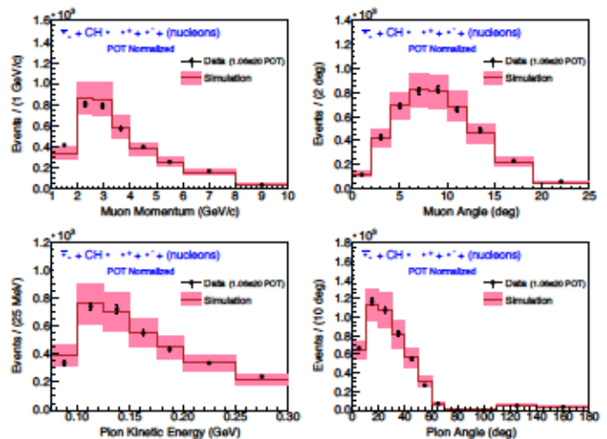
FIG. 4. Sideband sample distributions, MC versus data, for muon and pion kinematic variables (upper, lower plots respectively) prior to tuning of background and signal-contamination normalizations. The initial MC predictions and total systematic uncertainties are shown by the histograms and shaded error bands.
