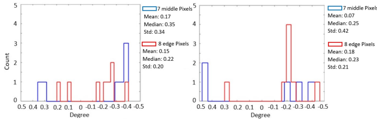
Fig. 6 Left : histogram of differential pointing of Pol A-Pol B in vertical axis, Right : histogram of differential pointing of Pol A-Pol B in horizontal axis for 7 middle and 8 edge antenna array pair. The Gaussian differential pointing values for both pairs are within the same values which indicates a smaller beam mismatch contributions from the corrugated frame. (Color figure online.)
