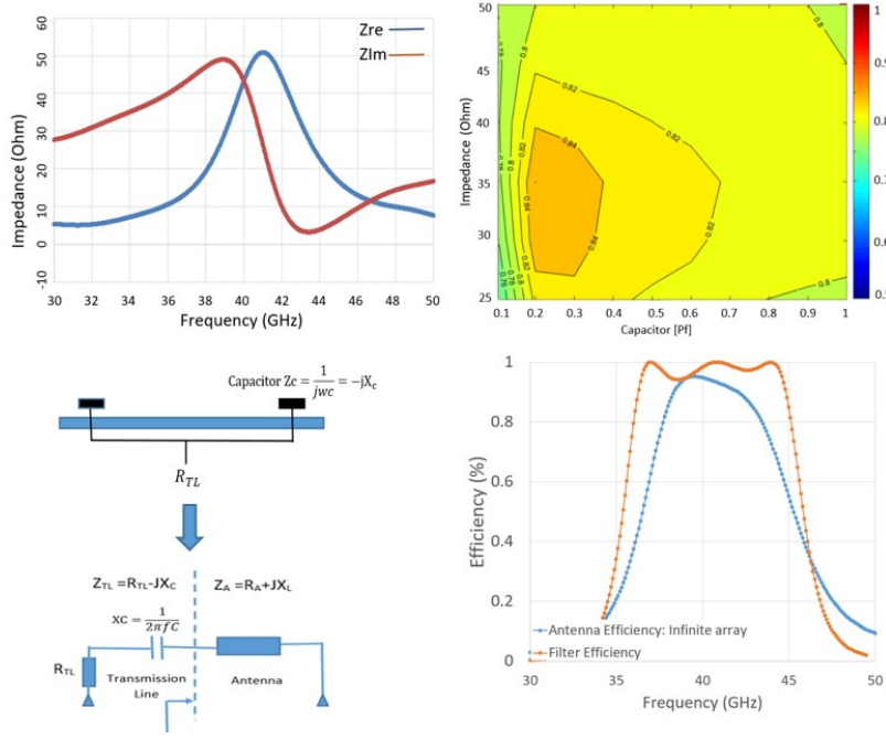
Fig. 2 Top/Left: The simulated real and imaginary impedance at the optimized feed point on the slot vs. frequency. Top/Right: The contour matching of the input microstrip impedance/capacitor to the antenna impedance. Bottom/Left: The equivalent matching circuit to the antenna. We used a series capacitor that shunt to ground to cancel out the inductive reactance impedance of the antenna. Bottom/Right: The expected antenna/filter efficiency versus frequency. The measured end to end Optical Efficiency (OE) is approximately between 30% to 36%. (Color figure online.)
