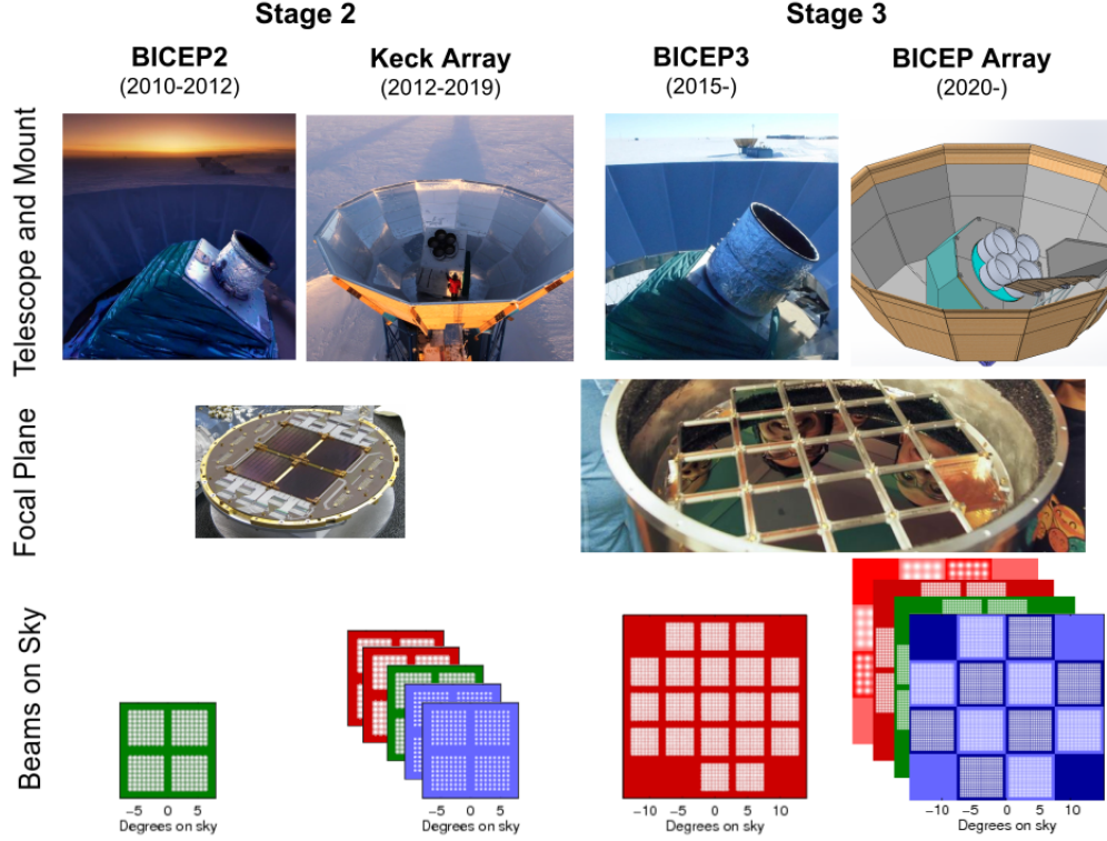
Figure 1: A graphical representation of the BICEP/Keck experiments from BICEP2 through BICEP Array. The middle and bottom rows show the increased focal plane size and density of the BICEP3 style receivers as compared to BICEP2 /Keck style. Different frequencies are represented in the bottom row by individual colors with the lowest frequency (30 GHz) visible in light red and the highest (270 GHz) visible in dark blue.
