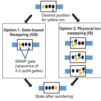
Fig. 5: Choices for chain reordering. GS uses a SWAP gate (implemented with 3 MS two-qubit gates) to exchange quantum state of any arbitrary pair of ions within the trap. IS requires hop-by-hop physical swaps.
