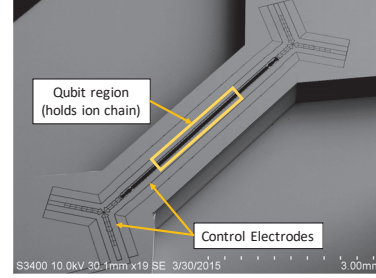
Fig. 1: Scanning electron micrograph of the Sandia HOA2 trap. Figure adapted from [24]. A single trap houses all the ions. Control electrodes are used to load, remove and move ions. This architecture does not scale beyond 50-100 qubits because of gate implementation challenges in long ion chains.
