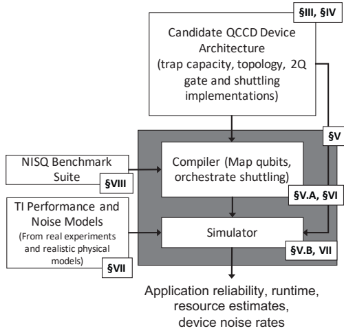
Fig. 3: Our framework for evaluating a candidate QCCD-based TI system. Taking a candidate architecture, a set of NISQ applications, and realistic performance models as input, the toolflow computes application metrics like runtime and reliability (fidelity) and device metrics like heating rates.
