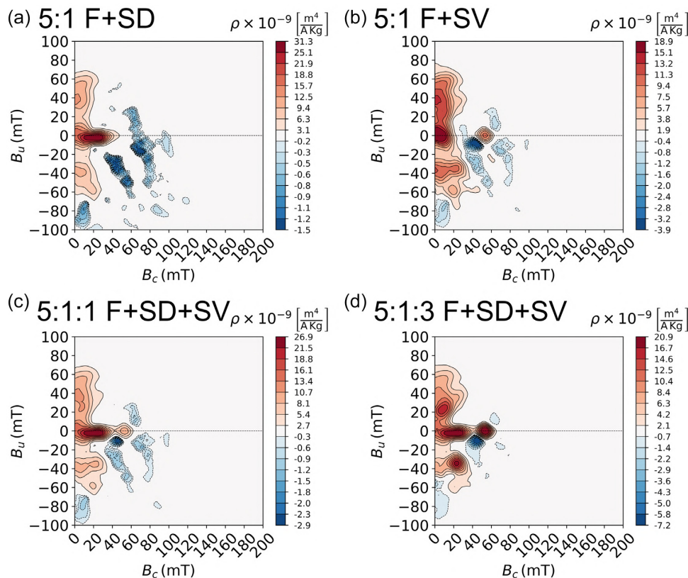
Figure 6. Simulated FORC diagrams for dispersions of framboids mixed with isolated particles. In (a) isolated particles are all in the SD size range (30–48 nm) and in (b) SV particles are modelled in the size range 70–80 nm. The framboidal (F), SD and SV simulations are mixed in varying proportions: (a) 5:1 F:SD, (b) 5:1 F:SV, (c) 5:1:1 F:SD:SV and (d) 5:1:3 F:SD:SV. SF = 2 in all FORC diagrams. The signal is dominated by the non-interacting particles because the framboidal signal is weaker per unit mass. The framboidal signal is still visible because it occupies regions that the isolated particles do not. Solutions for isolated particles are taken from Valdez-Grijalva et al. (2018a).
