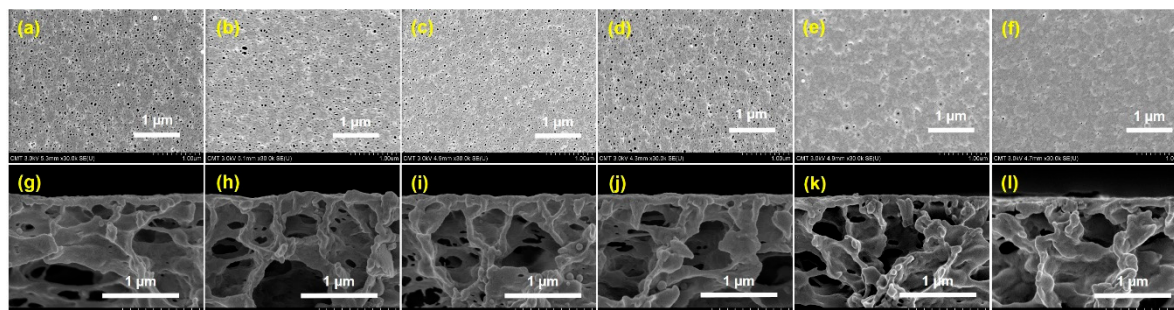
Figure 2. SEM images of surface and cross-section morphology for (a,g) PVDF, (b,h) PVDF-PSBMA 30s , (c,i) PVDF-PSBMA 60s , (d,j) PVDF-PSBMA 120s , (e,k) PVDF-PSBMA 180s , and (f,l) PVDF-PSBMA 300s .
