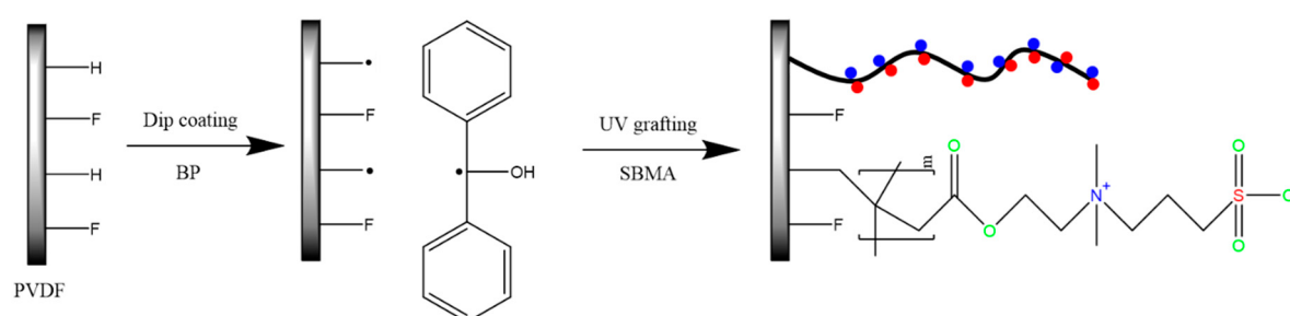
Scheme 1. The polyvinylidene difluoride (PVDF) modification of the sulfobetaine methacrylate (SBMA) monomer using the UV treatment polymerization process.
