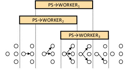
Figure 9: Active connections and bandwidth allocation change over time as transmissions start/end
