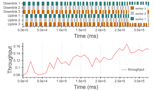
Figure 16: Distributed training of AlexNet with batch size of 8 and 3 workers on private CPU cluster. As downlinks/uplinks start interleaving, throughput increases.
