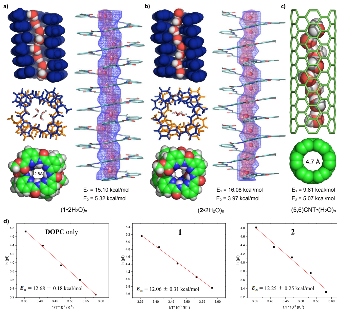
Figure 3. Water-containing crystal structures of 1 and 2 as well as computed structure of (5,6)CNT, the corresponding volume maps and the average binding energy between the wall interior and a water molecule from the water chain ( E_1 ) and average H-bond energy in the water chain ( E_2 ). a) Crystal structure of (1 \cdot 2H_2O)_n and energies of E_1 and E_2 calculated at the level of \omega B97X/6-31G++(2d,p) . b) Crystal structure of (2 \cdot 2H_2O)_n and energies of E_1 and E_2 . c) Water-containing structure of (5,6)CNT \cdot (H_2O)_n , having a cavity diameter of 4.7 Å, and energies of E_1 and E_2 . The pore volume maps (blue mesh) shown in a) and b) were obtained using the VolMap method in VMD in the format of 3D density grid (cubic grid size = 0.3 Å, diameter of the enclosing cylinder = 4.4 Å, grid densities of < 0.2 considered unoccupied). Using this method, the internal hollow cavity volume in (1 \cdot 2H_2O)_n estimatedly is > 20 vol% larger than that in (2 \cdot 2H_2O)_n . The volume maps (red) of the water chain (grid densities > 0.5 considered unoccupied) were also shown in a) and b). d) Arrhenius plots of the water permeability as a function of temperature (6° to 25°C) for DOPC only, 1 and 2 for determining activation energies ( E_a ) averaged over three runs.
