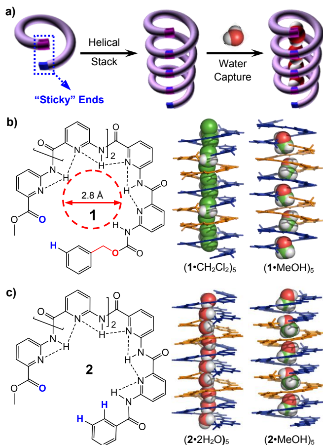
Figure 1. Molecular design and crystal structures of aquafolder-based synthetic water channels. a) A “sticky end”-mediated molecular strategy for creating self-assembled 1D nanotubes for water transport. b) Chemical and crystal structures of 1 , encapsulating 1D chain of dichloromethane ( \text{CH}_2\text{Cl}_2 ) or methanol ( \text{MeOH} ) 31 molecules. c) Chemical and crystal structures of 2 , encapsulating 1D chain of water or \text{MeOH} molecules. Sticky ends that are involved in forming intermolecular H-bonds are highlighted in blue.
