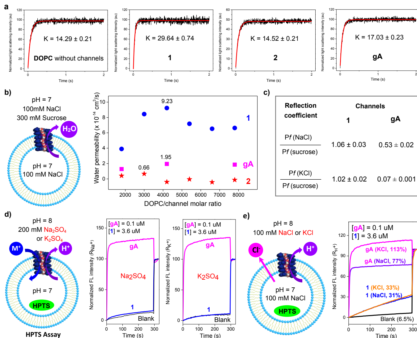
Figure 2. Water permeability of channels 1 , 2 and gA, and transport selectivity determined for 1 . a) Representative water transport curves for DOPC only, 1 , 2 and gA, obtained using a stopped flow apparatus at a lipid:channel molar ratio of 4200:1. Exponential coefficients (K) were obtained by fitting the data into the equation of y = A \cdot \exp(-kx) + y_0 . b) LUV-based hypertonic conditions (300 mM sucrose) for water permeability measurement for 1 , 2 and gA at different lipid:channel molar ratios, with data averaged in triplicate. c) Water permeability measured using three types of hypertonic conditions (300 mM sucrose, 250 mM NaCl or 250 mM KCl), suggesting complete and incomplete salt rejections by 1 and gA, respectively. d) HPTS-based LUV assays under high ionic concentration gradients, confirming that 1 does not transport both \text{Na}^+ and \text{K}^+ ions. e) HPTS-based LUV assays under a proton gradient, suggesting that (\text{I} \cdot 2\text{H}_2\text{O})_n is not optimized for transport of \text{Na}^+ or \text{K}^+ ions with respect to gA. Instead, it transports protons with slow passive diffusion of \text{Cl}^- to maintain the charge balance. gA = gramicidin A; HPTS = 8-Hydroxypyrene-1,3,6-trisulfonic acid.
