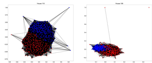
Fig. 3. PRAIME-RF output networks using 1-locfdr as the edge weights. Democrats are plotted as blue circles, and Republicans red triangles.
