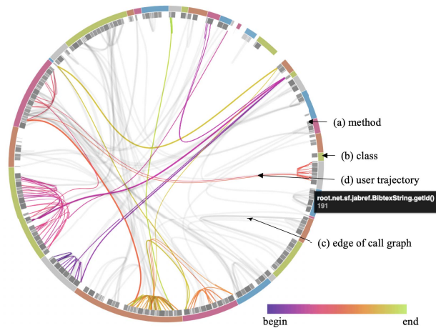
Fig. 2. An example of content space visualization. (a), each small box along the outer orbit represents a method, where details of the method are displayed on hover. (b), each arc along the orbit represents a class. (c), the gray curves are the edge bundling results of the call graph, where each edge connects a caller and a callee. (d), the color curve corresponds to a user trajectory. The color scalar indicates the scanning sequences.
