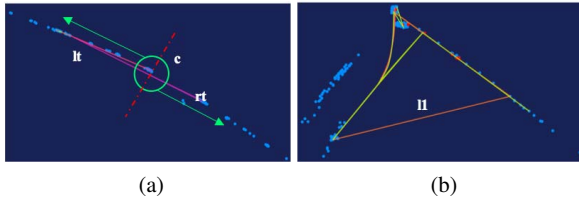
Fig. 14. Flag patterns from the tree graph (a) and the call graph (b). In (a), we identify three patterns, lt for left, c for center, and rt for right. In (b), we identify a line ll that appears frequently among the trajectories.
