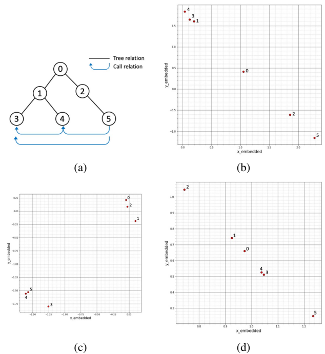
Fig. 3. A simple example of embedding a graph (a) into 2D space according to (b) the tree, (c) the call graph, and (d) the combination of the tree and the call graph.
