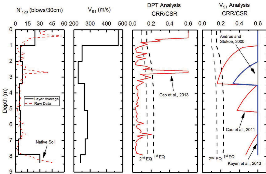
Figure 5. (a) DPT blowcount vs. depth; (b) V_{s1} vs. depth, and (c) CRR/CSR ratio for DPT and (d) shear wave velocity procedures in Argostoli port.
