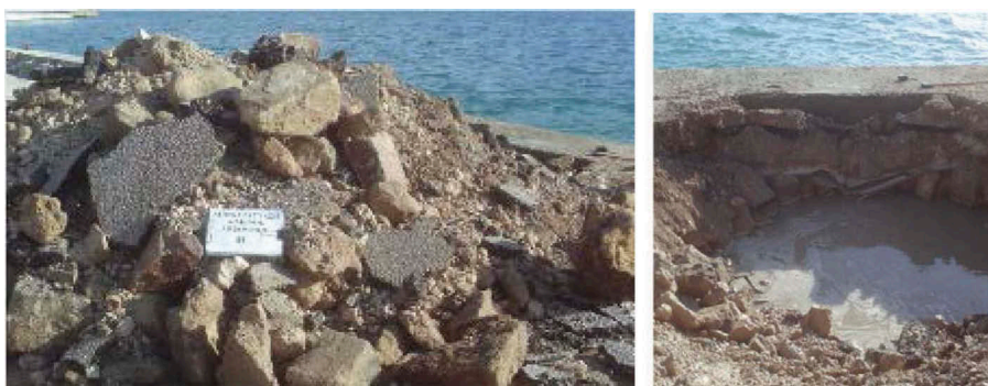
Figure 4. Views of debris excavated adjacent to the port seafront at the location where the maximum lateral displacement of the quay walls was registered in Lixouri. The large particles of the fill material is visible. (Geoconsult Ltd, 2016)
