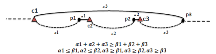
Figure 8: Upper bound of approximation factor
