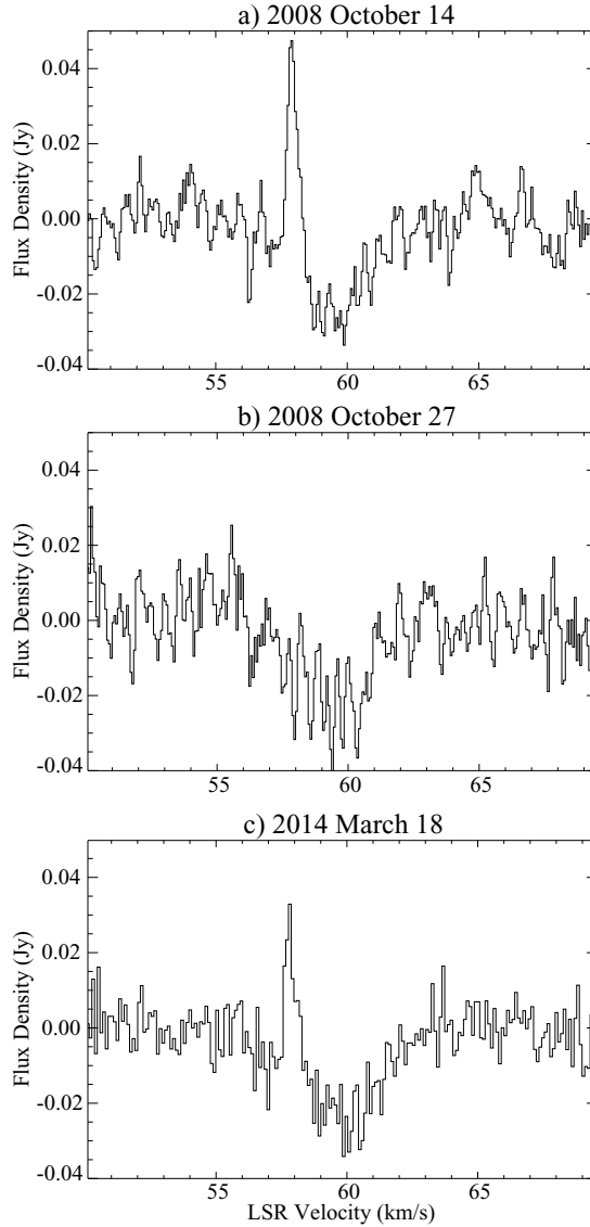
Figure 2. CH 3 OH spectra of the 6.7 GHz transition toward G45.12+0.13 obtained in three epochs: a) 2008 October 14; b) 2008 October 27; c) 2014 March 18. Note the detection of a variable recurrent maser; as explained in section 3, the line could be caused by detection of the strong maser in G45.07+0.13 in a sidelobe of the telescope. The data shown in the figure are available as supplemental online material.
