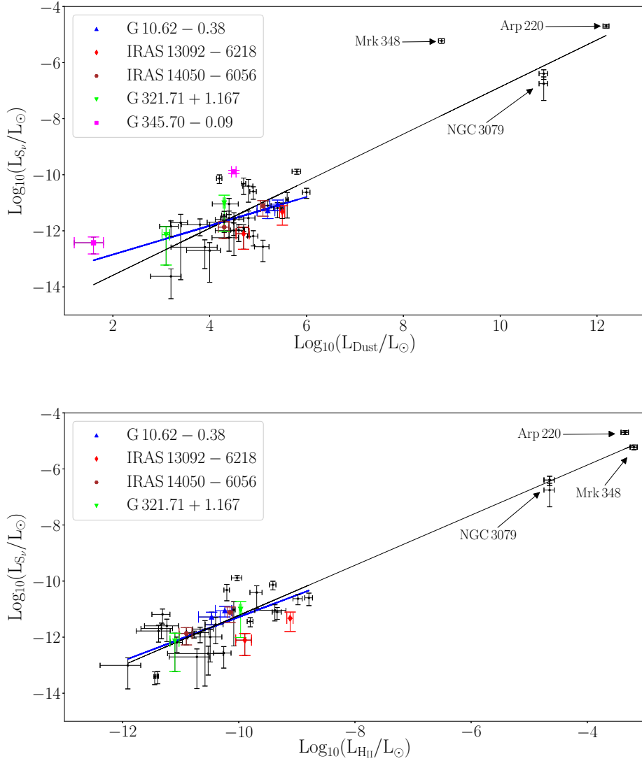
Figure 8. Absorption luminosity of the 6.7 GHz \text{CH}_3\text{OH} line ( L_{S_\nu} = 4\pi|S_{\nu,\text{line}}|d^2 ) as a function of FIR luminosity ( upper panel ) and 5 GHz radio luminosity ( lower panel ). Sources identified with different symbols and colours are regions for which the distance ambiguity has not been resolved, and thus, significantly different luminosity values are possible. No interferometric continuum observations of G345.70–0.09 are available, thus, it was not included in the lower panel . All data in the upper panel were fit with an \alpha = 0.84 \pm 0.07 power law (black fit); the thick slope (blue line) shows the fit ( \alpha = 0.51 \pm 0.14 ) when the extragalactic sources are excluded. The data in the lower panel were also fit with a power-law ( \alpha = 0.89 \pm 0.05 ) when all data are included (black fit), and with a power-law \alpha = 0.78 \pm 0.16 when only sources with \log(L_{\text{HI}}/L_\odot) between -12 and -8 are included (thick fit line shown in blue).
