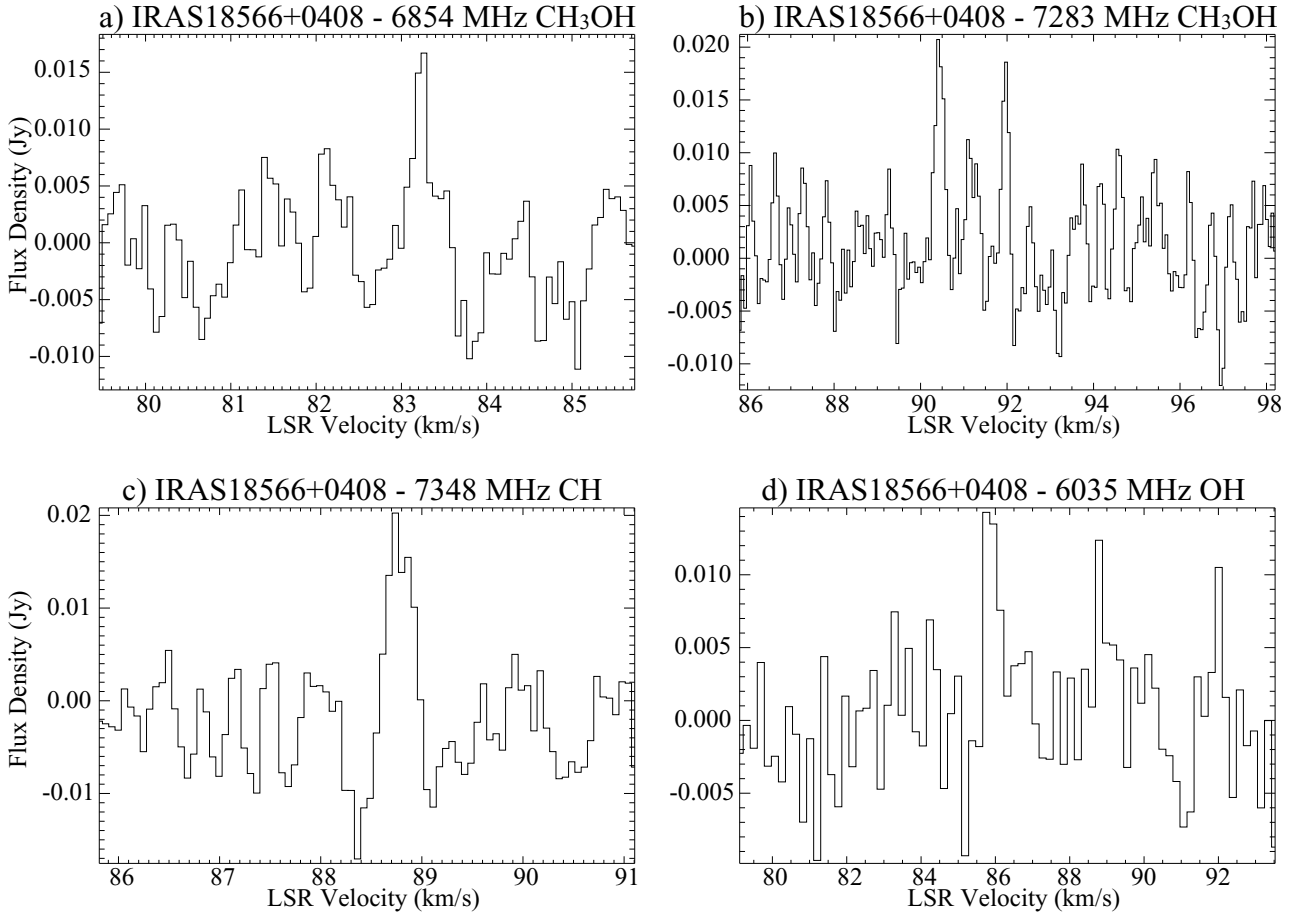
Figure 6. Spectra of weak lines toward IRAS 18566+0408. Panels a), b), and c) show tentative detections, while the weak line shown in panel d) is a confirmed 6.035 GHz OH detection, as Al-Marzouk et al. (2012) reported this line and showed that the line is highly variable, possibly correlated with the variability of 6.7 GHz CH 3 OH masers in the region. The tentative detections were not confirmed in the follow-up observations (Table 3), thus the lines may be variable or artefacts. The data shown in the figure are available as supplemental online material.
