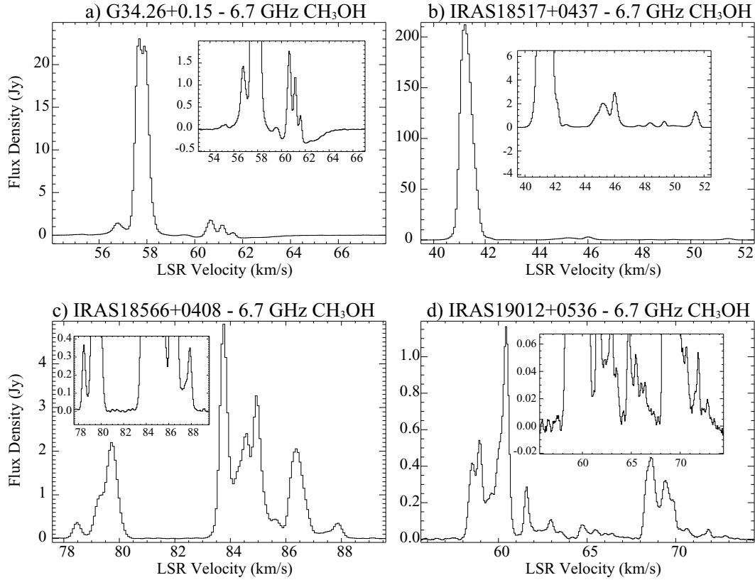
Figure 1. Detection of CH 3 OH lines toward eight sources (see Table 5; the G45.12+0.13 spectra is shown in Figure 2). Insets highlight weak masers and/or absorption. The data shown in the figure are available as supplemental online material.
