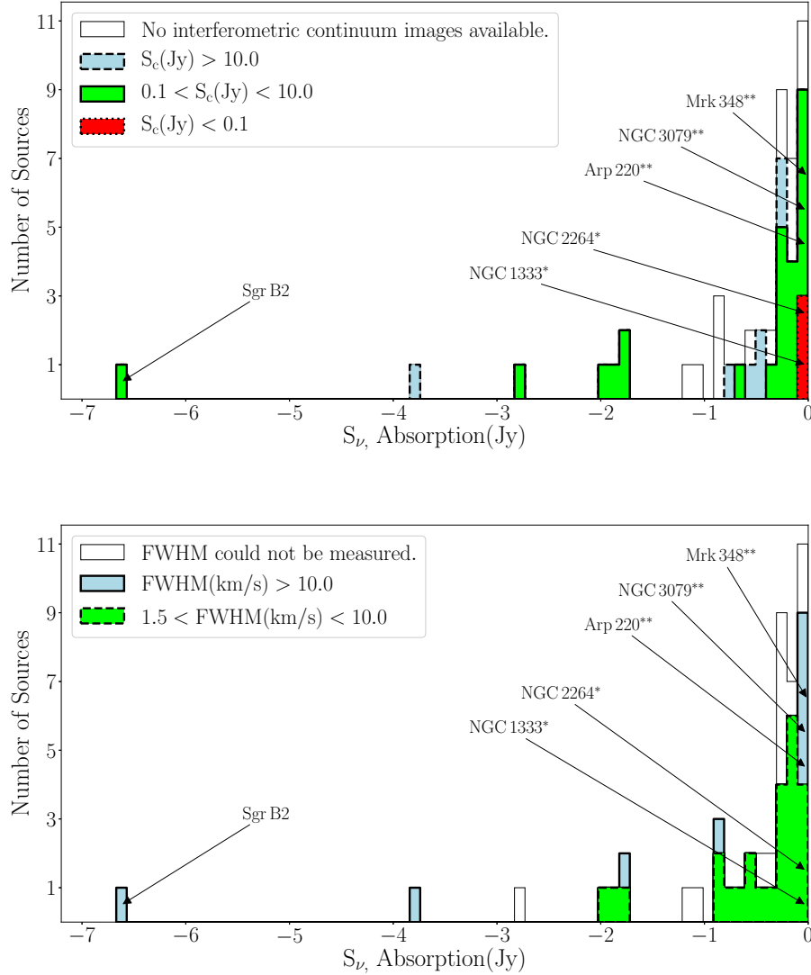
Figure 7. Histogram of the number of sources with 6.7 GHz methanol absorption at different flux density bins. Colours and line type (solid, dashed, dotted) in the upper panel identify the radio continuum flux density based on interferometric images. Colours and line type in the lower panel identify ranges in FWHM of the absorption lines. (*) NGC 1333 is a low-mass star forming region and the absorption is against the CMB (Pandian et al. 2008). The absorption line detected toward NGC 2264 is also likely against the CMB (Pandian et al. 2008). (**) Extragalactic absorption has been reported toward NGC 3079, Arp 220 and Mrk 348.
