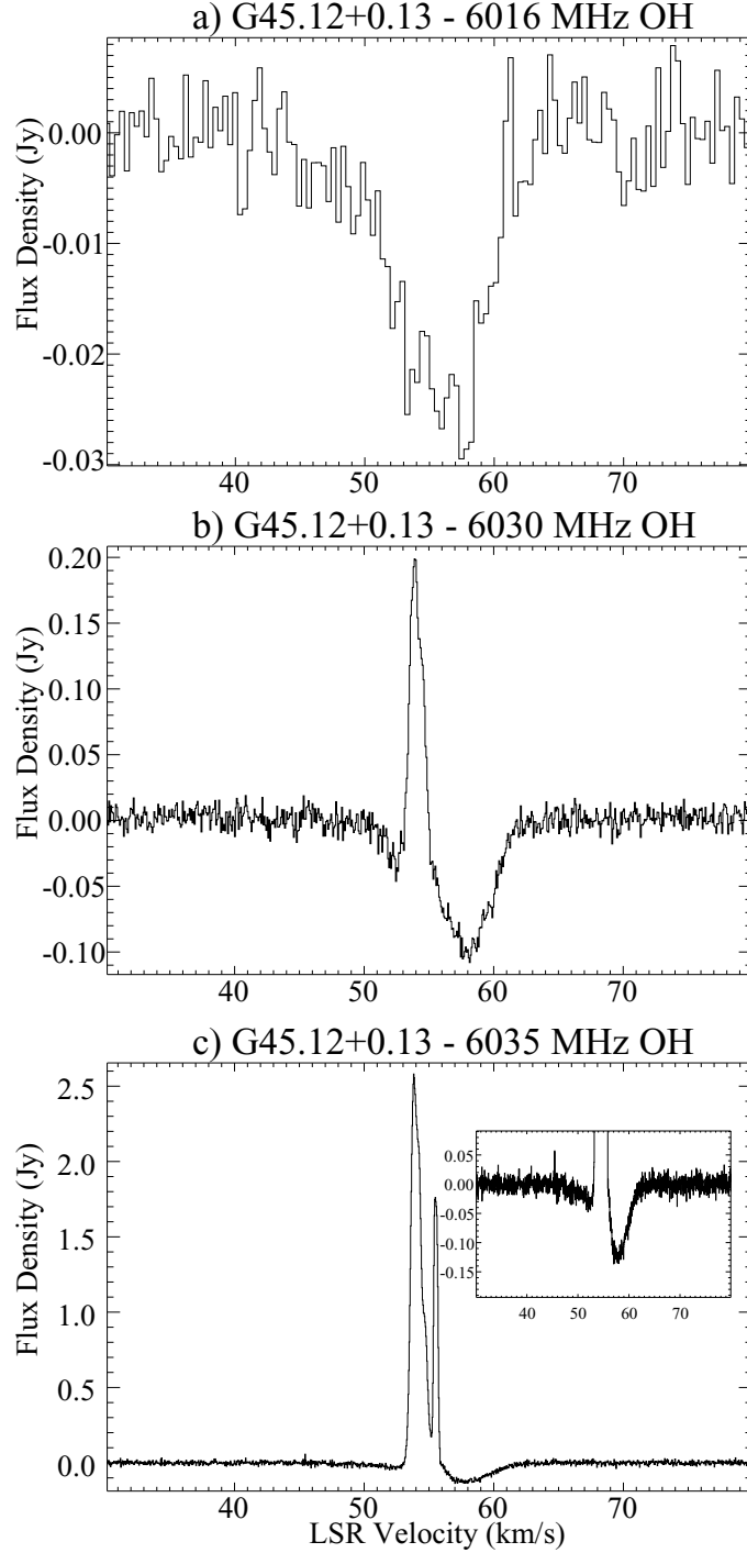
Figure 4. Detection of excited OH lines toward G45.12+0.13 at three different frequencies (see Tables 3, 6, 8). The inset in the bottom panel shows a zoom-in view of the absorption line. The data shown in the figure are available as supplemental online material.
