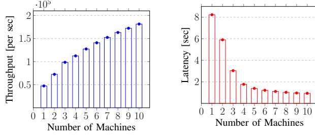
Fig. 6: Measuring (a) Throughput and (b) Latency with varying the number of machines
