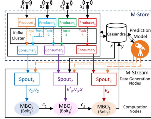
Fig. 3: M-DB Implementation over Apache Storm and Kafka
