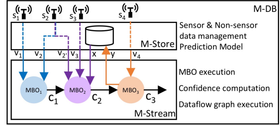
Fig. 1: M-DB Architecture
