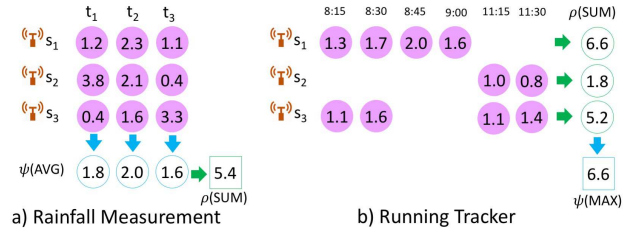
Fig. 2: Two Applications of Spatio-temporal Operators
