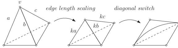
FIGURE 1. Discrete conformal change of PL metrics. All triangulations are Delaunay
