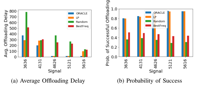
Fig. 5: Performance Under Different Signal Settings
