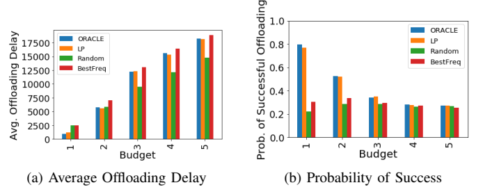
Fig. 4: Performance Under Different Budgets
