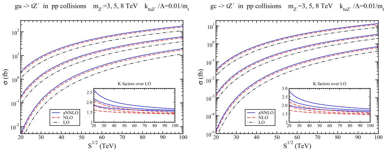
Fig. 9 Total cross sections for the (left) gu \rightarrow tZ' and (right) gc \rightarrow tZ' processes with anomalous couplings. The plots show results as a function of collider energy for three choices of Z' mass, 3, 5, and 8 TeV. The inset plots display K -factors. CT14NNLO PDFs are used
