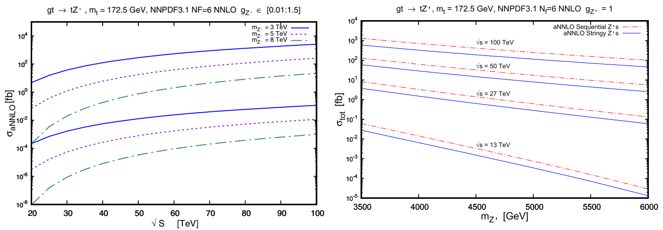
Fig. 19 Left: Scan of the g_{Z'} parameter for the gt \rightarrow tZ' process. The plot shows results of the total cross section at aNNLO as a function of collider energy. Bands with different dashed represent Z' mass values
