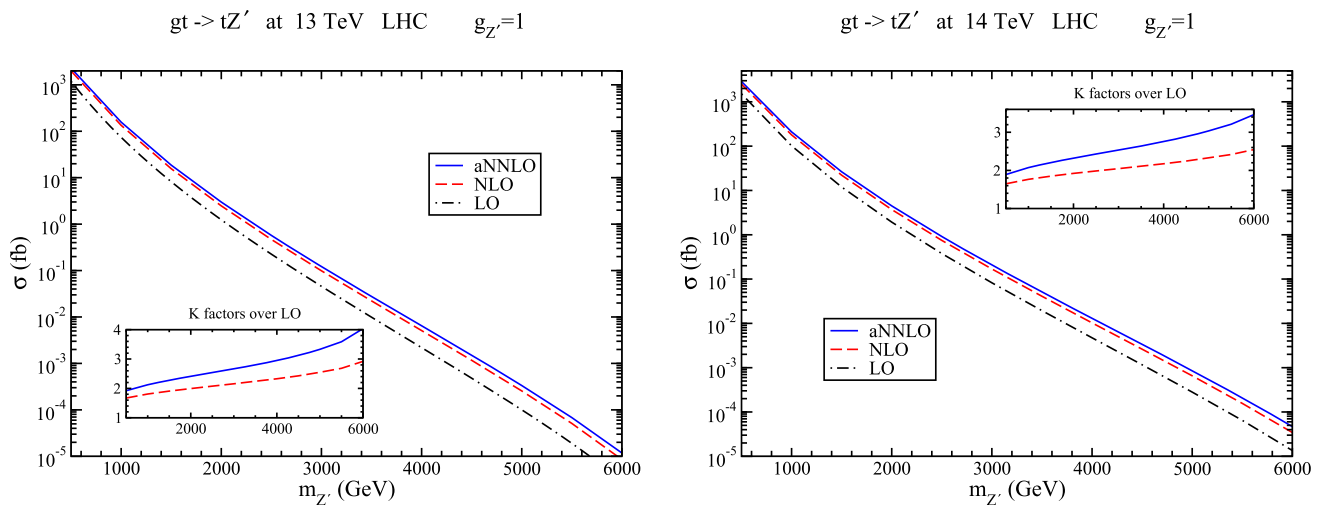
Fig. 20 Total cross section for the gt \rightarrow tZ' process at the LHC 13 TeV (left) and 14 TeV (right). LO, NLO and NNLO calculations are obtained using NNPDF3.1 NNLO n_f = 6 PDFs
