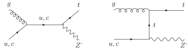
Fig. 1 Leading-order diagrams for gu \rightarrow tZ' with anomalous t-u-Z' coupling and gc \rightarrow tZ' with anomalous t-c-Z' coupling
