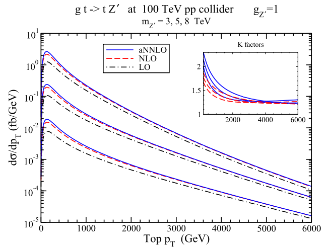
Fig. 23 Top-quark p_T distributions for the gt \rightarrow tZ' process at 100 TeV pp collider energy for m_{Z'} = 3, 5 , and 8 TeV. NNPDF3.1 NNLO n_f = 6 PDFs are used for LO, NLO, and aNNLO calculations
