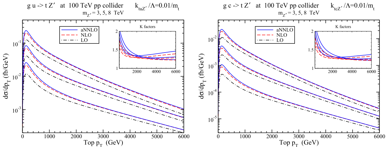
Fig. 11 Top-quark p_T distributions for the (left) gu \rightarrow tZ' and (right) gc \rightarrow tZ' processes with anomalous couplings for m_{Z'} = 3, 5 , and 8 TeV at 100 TeV pp collider energy. Inset plots: NLO/LO and aNNLO/LO K-factors. CT14NNLO PDFs are used
