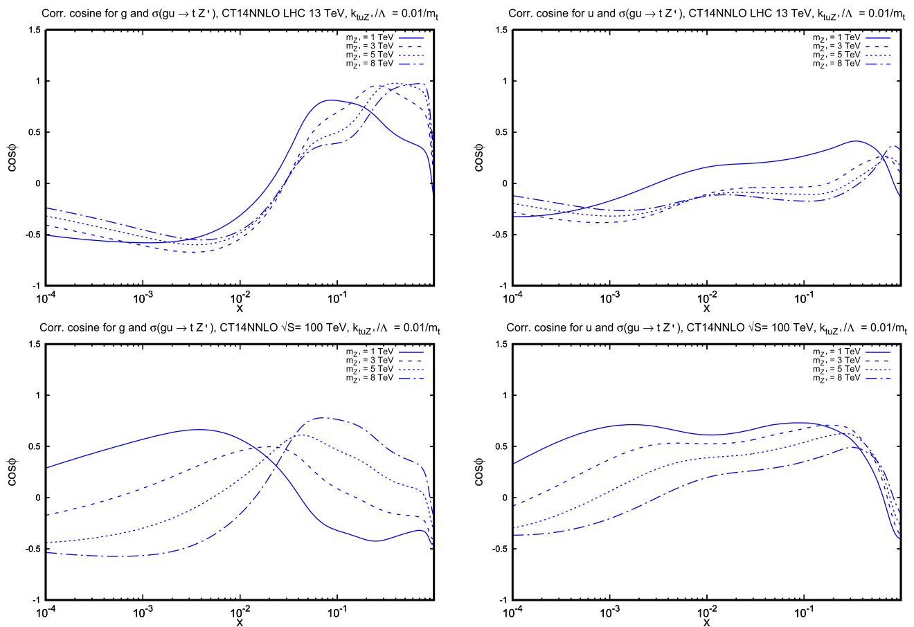
Fig. 12 Correlation cosine at \sqrt{S}=13 and 100 TeV between \sigma_{gu \rightarrow tZ'} and the gluon as a function of x_{\text{gluon}} (left column) and \sigma_{gu \rightarrow tZ'} and the up-quark as a function of x_{\text{up}} (right column). The four panels show aNNLO results rescaled at the 68% C.L. for different values of the Z' mass
