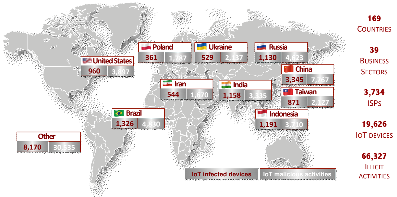
Fig. 7. Global distribution of exploited IoT devices
