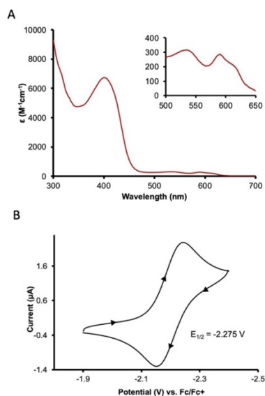
Figure 3. Characterization data for Co II (BQN) 2 ( 1 ). (A) UV-visible absorption spectrum in CH 2 Cl 2 , inset: d-d transitions, and (B) cyclic voltammogram, scan rate 100 mV/sec with 0.1M TBAPF 6 as the supporting electrolyte in CH 3 CN. Referenced vs. Fc/Fc + .
