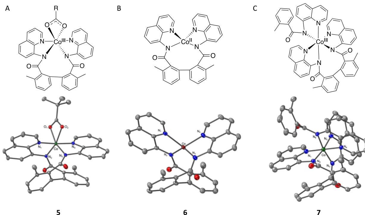
Figure 13. 2D and thermal ellipsoid diagrams of the single-crystal structures of complexes (PivO)Co III (BQN-BQN), ( 5 ), Co II (BQN-BQN), ( 6 ), and (BQN)Co III (BQN-BQN), ( 7 ). 50% ellipsoid probability; H-atoms omitted for clarity. Complex 5 select distances: Co–N 1 , 1.913 Å; Co–N 2 , 1.940 Å; Co–N 3 , 1.918 Å; Co–N 4 , 1.917 Å; Co–O 1 , 1.977 Å; Co–O 2 , 1.969 Å. Complex 6 select distances: Co–N 1 , 2.029 Å; Co–N 2 , 1.971 Å; Co–N 3 , 1.972 Å; Co–N 4 , 2.027 Å. \tau_4 = 0.726 . Complex 7 select distances: Co–N 1 , 1.920 Å; Co–N 2 , 1.998 Å; Co–N 3 , 2.004 Å; Co–N 4 , 1.937 Å; Co–N 5 , 1.993 Å; Co–N 6 , 1.951 Å.
