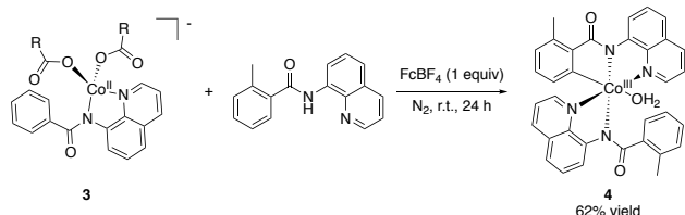
Scheme 4. Oxidation of Complex 2 to form the C–H Bond Activated Co(III) Complex, 4 , with a Co–C bond
