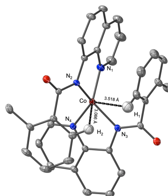
Figure 2. Thermal ellipsoid plot of Co II (BQN) 2 , ( 1 ). Ellipsoids drawn at 50% probability; H-atoms have been omitted for clarity with exception of H 1 and H 2 showing the intramolecular Co–H distances. Select distances (in parentheses are given the calculated values): Co–N 1 : 2.023 (2.06) Å; Co–N 2 : 1.967 (2.00) Å; Co–N 3 : 1.967 (2.00) Å; Co–N 4 : 2.024 (2.06) Å. Select angles: N 1 –Co–N 2 : 83.1°; N 1 –Co–N 4 : 119.9°; N 3 –Co–N 4 : 82.9°; N 2 –Co–N 4 : 122.1°.
