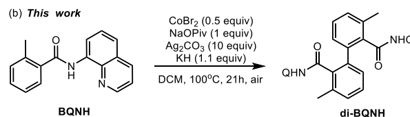
Scheme 1. Representative of the Cobalt-Mediated Dehydrogenative Dimerization of Aminoquinoline Benzamide Derivatives.
