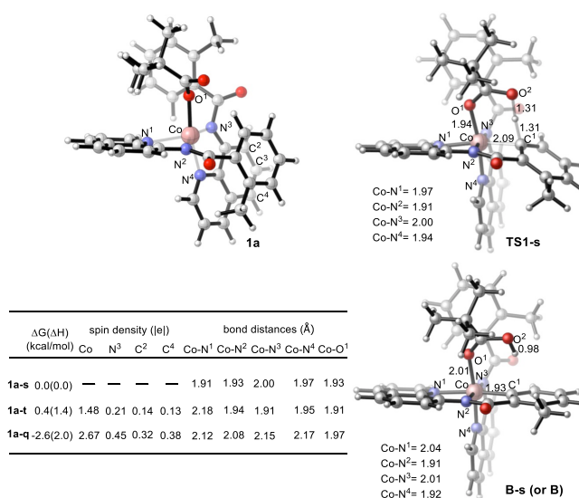
Figure 7. Relative energies, spin density distribution, and important geometry parameters of the singlet, triplet, and quintet states of the complex (PivO)Co(BQN) 2 , 1a , as well as geometry parameters of the first C–H deprotonation transition state TS1-s and product B-s .
