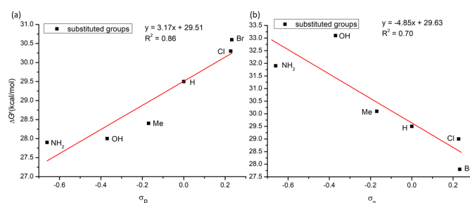
Figure 12. Linear correlation between activation barrier and Hammett parameter ( \sigma_p ) of the used substituents. (a) para -substituted aryl group; (b) para -substituted pyridine of the AQ ligand.
