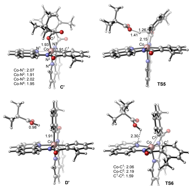
Figure 11. Geometries and spin densities of key intermediates and transition states (bond distances are given in Å) of anionic pathway of the studied Co-mediated dehydrogenative aminoquinoline directed benzamide dimerization.
