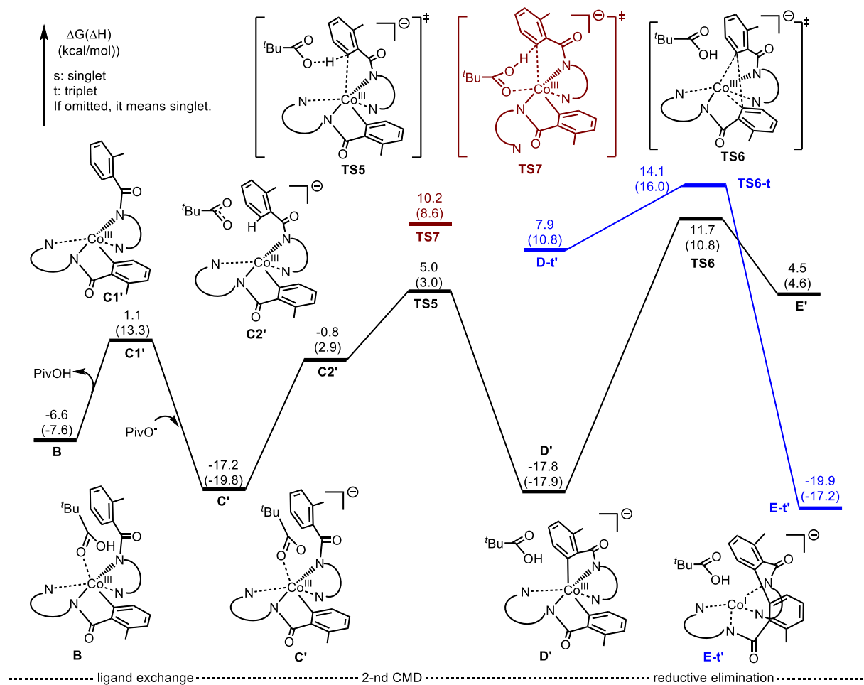
Figure 10. Potential energy surface for the anionic mechanism of the Co-mediated dehydrogenative aminoquinoline directed benzamide dimerization.
