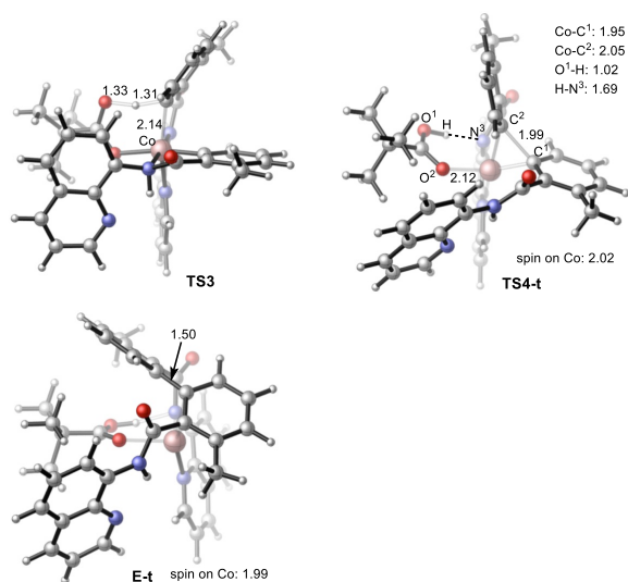
Figure 9. Geometries and spin densities of key transition states and product (bond distances are given in Å) of charge neutral pathway of the Co-mediated dehydrogenative dimerization of aminoquinoline directed benzamides.
