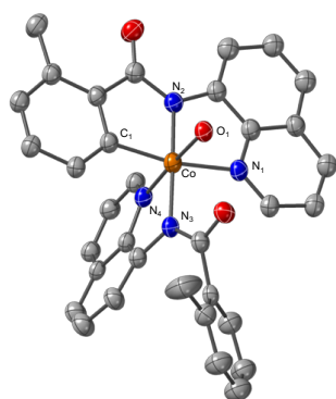
Figure 6. ORTEP diagram of complex 4 . 50% ellipsoid probability; H atoms omitted for clarity. Select distances are: Co–C 1 , 1.928 Å; Co–N 1 , 2.029 Å; Co–N 2 , 1.893 Å; Co–N 3 , 1.903 Å; Co–N 4 , 1.982 Å; Co–O 1 , 1.959 Å.
