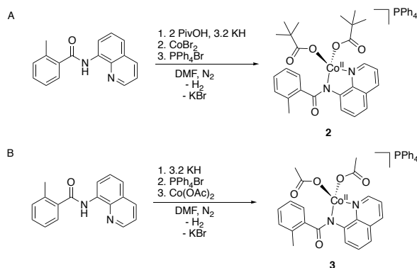
Scheme 3. Synthesis of the Carboxylate and Aminoquinoline Containing Complexes (A) PPh 4 [Co II (BQN)(PivO) 2 ] ( 2 ), and (B) PPh 4 [Co II (BQN)(OAc) 2 ] ( 3 )
