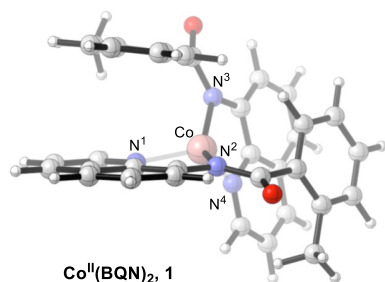
Figure 1. The calculated structure of initial intermediate Co II (BQN) 2 , 1 . For its selected geometry parameters, see Figure 2, as well as Supporting Information.
