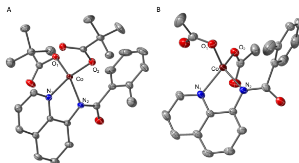
Figure 4. ORTEP diagrams of the single-crystal structures of (A) complex 2 and (B) complex 3 . 50% ellipsoid probability; H atoms omitted for clarity. Select distances are: for complex 2 , Co–N 1 , 2.035 Å; Co–N 2 , 2.006 Å; Co–O 1 , 1.954 Å; Co–O 2 , 1.950 Å, and for complex 3 , Co–N 1 , 2.043 Å; Co–N 2 , 2.016 Å; Co–O 1 , 1.993 Å; Co–O 2 , 1.952 Å.
