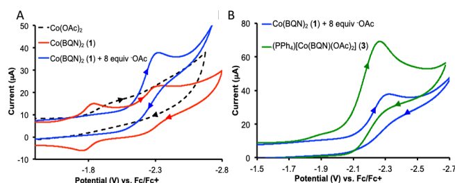
Figure 5. Cyclic voltammogram of A) Co II (BQN) 2 ( 1 ) titrated with additional acetate and B) an overlay of the cyclic voltammogram of isolated PPh 4 [Co II (BQN)(OAc) 2 ] ( 3 ) with the acetate titration of Co II (BQN) 2 ( 1 ). Scan rate of 100 mV/sec, with 0.1 M TBAPF 6 as the supporting electrolyte in dimethylformamide (DMF). Referenced vs. Fc/Fc + .
