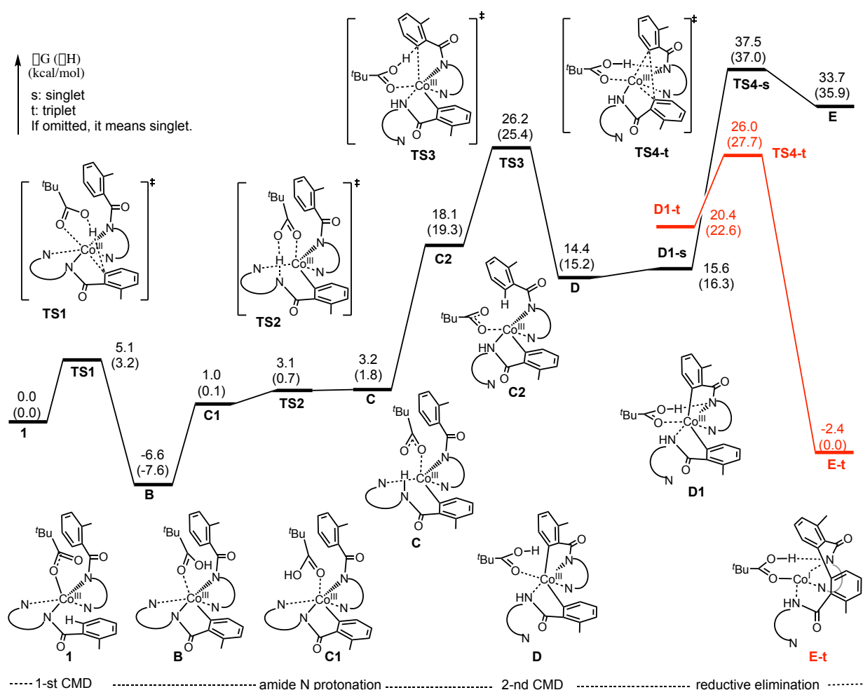
Figure 8. Potential energy surface for the charge neutral pathway of the Co-mediated dehydrogenative dimerization of aminoquinoline directed benzamides.
