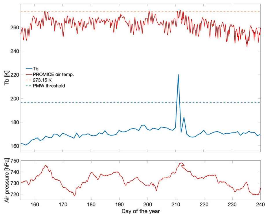
Figure 4. Time series of daily air temperature (top red line) recorded at the EGP PROMICE station ( 75.6247^{\circ}\text{N} , 35.9748^{\circ}\text{W} , 2660 m a.s.l.) together with time series of spaceborne brightness temperatures at 19.35 GHz recorded over the pixel containing the location of the EGP station (blue line) together with air pressure (hPa) recorded at the same station (bottom red line). The dashed orange line represents the 273.15 K values, and the blue dashed line represents the threshold on Tb above which melting is considered to occur.
