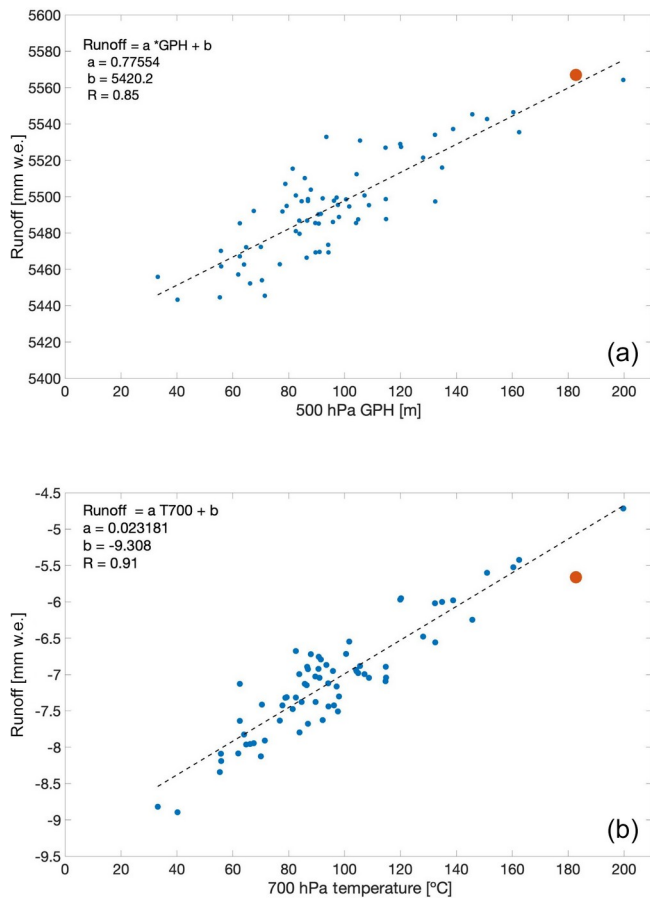
Figure 13. Scatterplot between runoff (mm w.e.) and (a) 500 hPa GPH (m) and (b) 700 hPa temperature (°C). Red disks show 2019 values in both plots. The coefficient of a linear regression analysis are reported within each plot, together with the coefficient of determination R .
