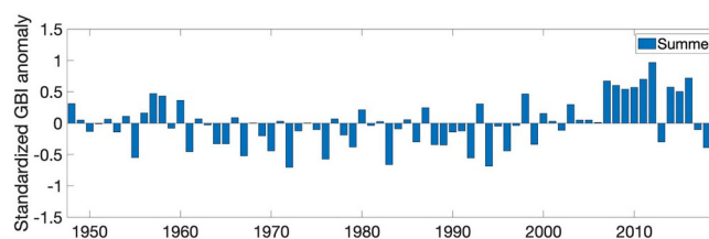
Figure 12. Standardized (1981–2010) (a) summer (JJA) averaged GBI values for the period 1948–2019.
