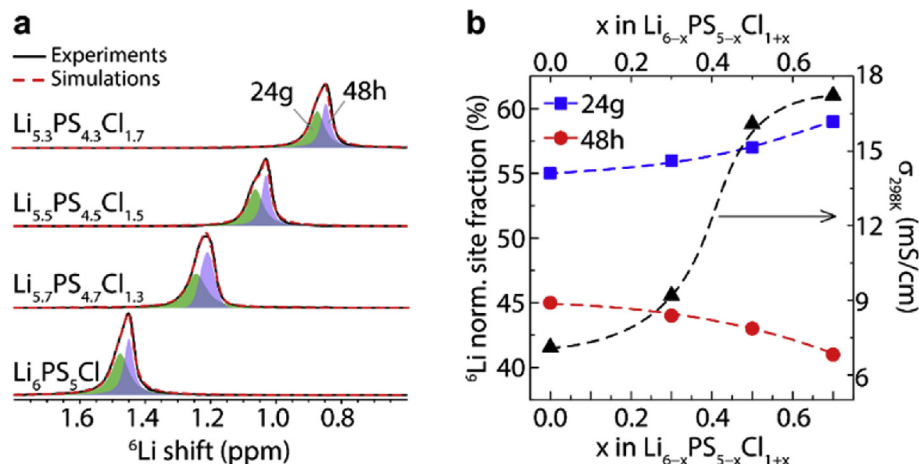
Fig. 4. Li site occupancy in \text{Li}_{6-x}\text{PS}_{5-x}\text{Cl}_{1+x} ( x = 0, 0.3, 0.5 , and 0.7 ) probed by solid-state ^6\text{Li} NMR: (a) ^6\text{Li} magic-angle-spinning (MAS, 25 kHz) NMR spectra. (b) Normalized Li site fractions and ionic conductivity in \text{Li}_{6-x}\text{PS}_{5-x}\text{Cl}_{1+x} ( x = 0, 0.3, 0.5 , and 0.7 ).
