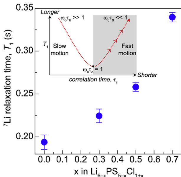
Fig. 5. ^7\text{Li} NMR T_1 relaxation time of \text{Li}_{6-x}\text{PS}_{5-x}\text{Cl}_{1+x} ( x = 0, 0.3, 0.5 , and 0.7 ) as an indicator of ion mobility.
