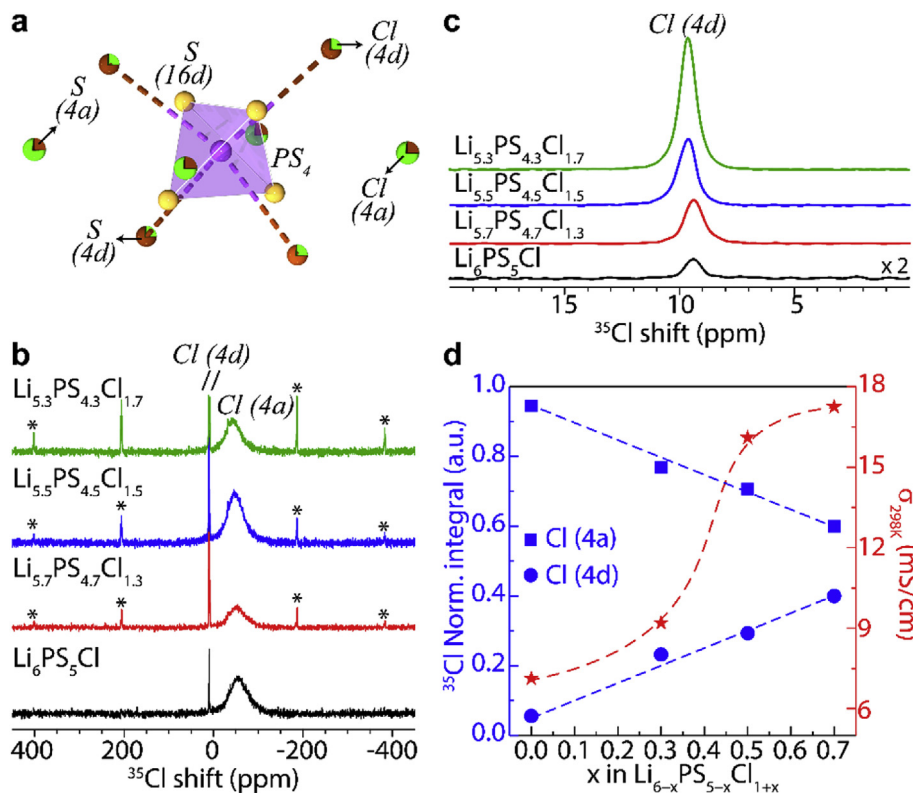
Fig. 7. (a) The schematic of S^{2-}/Cl^{-} mixing at 4d/4a sites. ^{35}Cl NMR spectra showing the Cl (4a) resonance (b) and the Cl (4d) resonance site (* denoting the spinning side bands of the Cl (4d) resonance) (c) in Li_{6-x}PS_{5-x}Cl_{1+x} , x = 0, 0.3, 0.5 , and 0.7 . (d) The correlation of ionic conductivity with the normalized ^{35}Cl NMR integrals as a function of Cl content.
