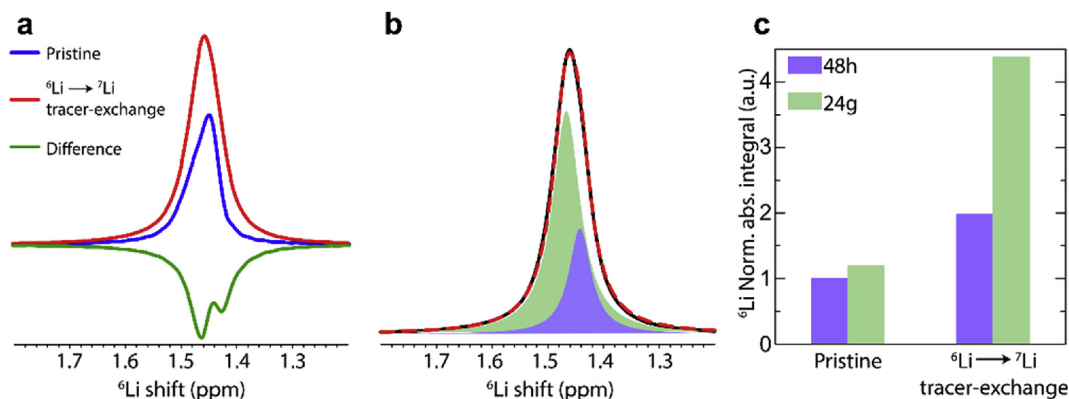
Fig. 8. Detection of ion transport pathways in \text{Li}_6\text{PS}_5\text{Cl} with ^6\text{Li} \rightarrow ^7\text{Li} tracer-exchange NMR: (a) ^6\text{Li} NMR spectra before/after tracer exchange. The difference spectrum shows both Li sites are ^6\text{Li} enriched. (b) Simulation results of the ^6\text{Li} NMR spectrum after ^6\text{Li} \rightarrow ^7\text{Li} tracer-exchange. Red dashed line denotes the simulation. (c) Comparisons of Li site fractions before/after ^6\text{Li} \rightarrow ^7\text{Li} tracer-exchange. The ^6\text{Li} NMR integrals are normalized based on the ^6\text{Li} (48h) integral in pristine \text{Li}_6\text{PS}_5\text{Cl} . (For interpretation of the references to colour in this figure legend, the reader is referred to the web version of this article).
