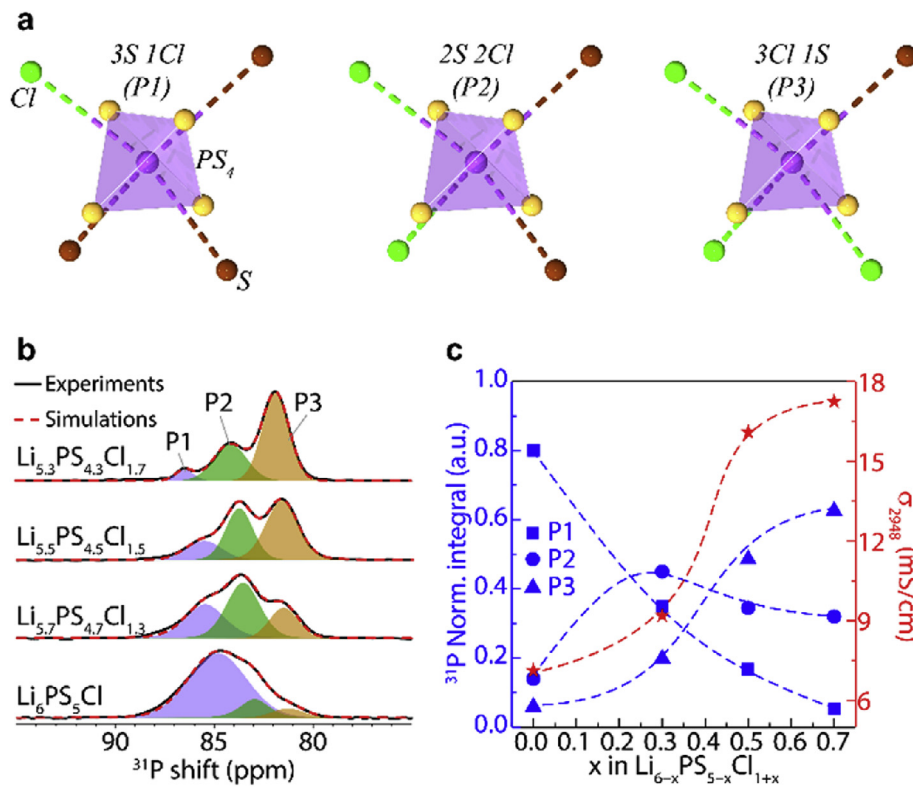
Fig. 6. (a) The schematic of distinct P environments induced by different levels of S^{2-}/Cl^{-} mixing at 4d/4a sites. (b) ^{31}P NMR spectra of Li_{6-x}PS_{5-x}Cl_{1+x} , x = 0, 0.3, 0.5 , and 0.7 . (c) The ionic conductivity and the normalized ^{31}P integral of P1, P2, and P3 NMR resonances as a function of x in Li_{6-x}PS_{5-x}Cl_{1+x} .
