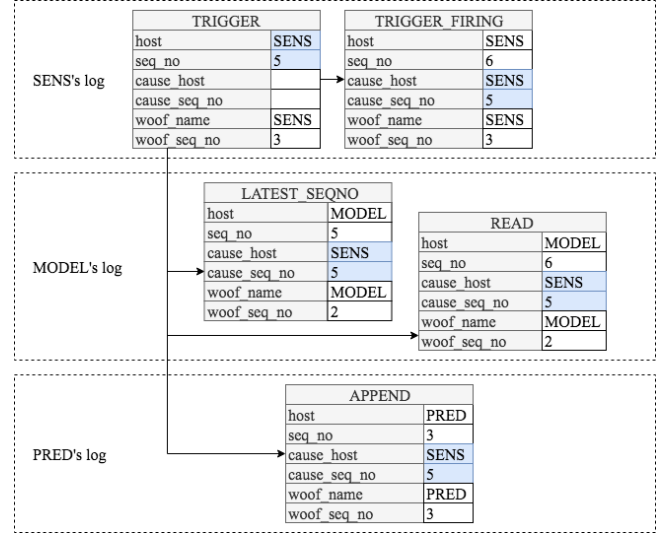
Figure 3: CSPOT namespace log events from the Sensor repair example.
