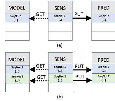
Figure 1: Data repair example. Application state is stored in persistent, append-only data structures (SENS, MODEL, and PRED) on 1+ hosts; each version has a sequence number (SeqNo). (a) shows the state after the first sensor element arrives; (b) shows the state after a second sensor element.
