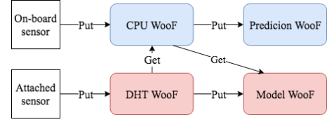
Figure 5: The Temperature prediction application structure
