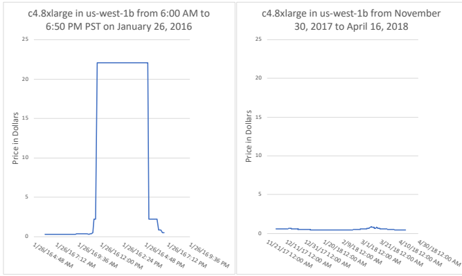
Fig. 1: Both figures show price time series data for the same c4.8xlarge instance type in us-west-1b . On the left we present a short window from 6:00 AM PST 6:50 PM PST on January 26, 2016 before the switch to retail pricing. On the right we show the window after the switch to retail pricing from November 30, 2017 and ends at approximately 4:00 PM PST on April 16, 2018
