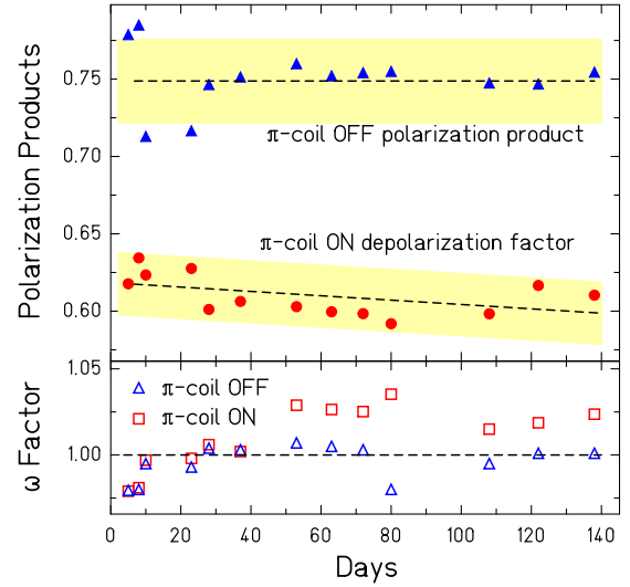
FIG. 3. The upper plot shows the average of the west and east polarimeter polarization products PA with the \pi coil off and corresponding depolarization factors d when the \pi coil was on [65]. The error bars on individual points represent one-sigma, statistical uncertainties; shaded bands show average errors per point based on their means. The lower plot gives \omega^0 (triangles) and \omega^\pi (squares), the fraction by which each side differs from the average for polarization products and depolarizations respectively.
