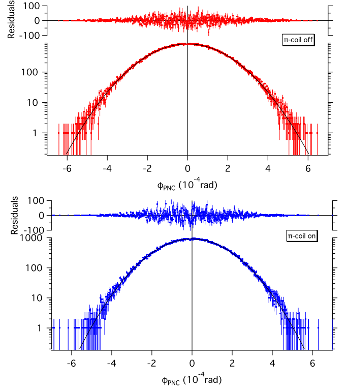
FIG. 7. Distribution of measured spin rotation angles in liquid ^4\text{He} with \pi coil off (upper plot) and \pi coil on (lower plot). The error bars represent one-sigma statistical uncertainty. The solid lines are fits to a Gaussian function, and the residuals are shown above the data.
