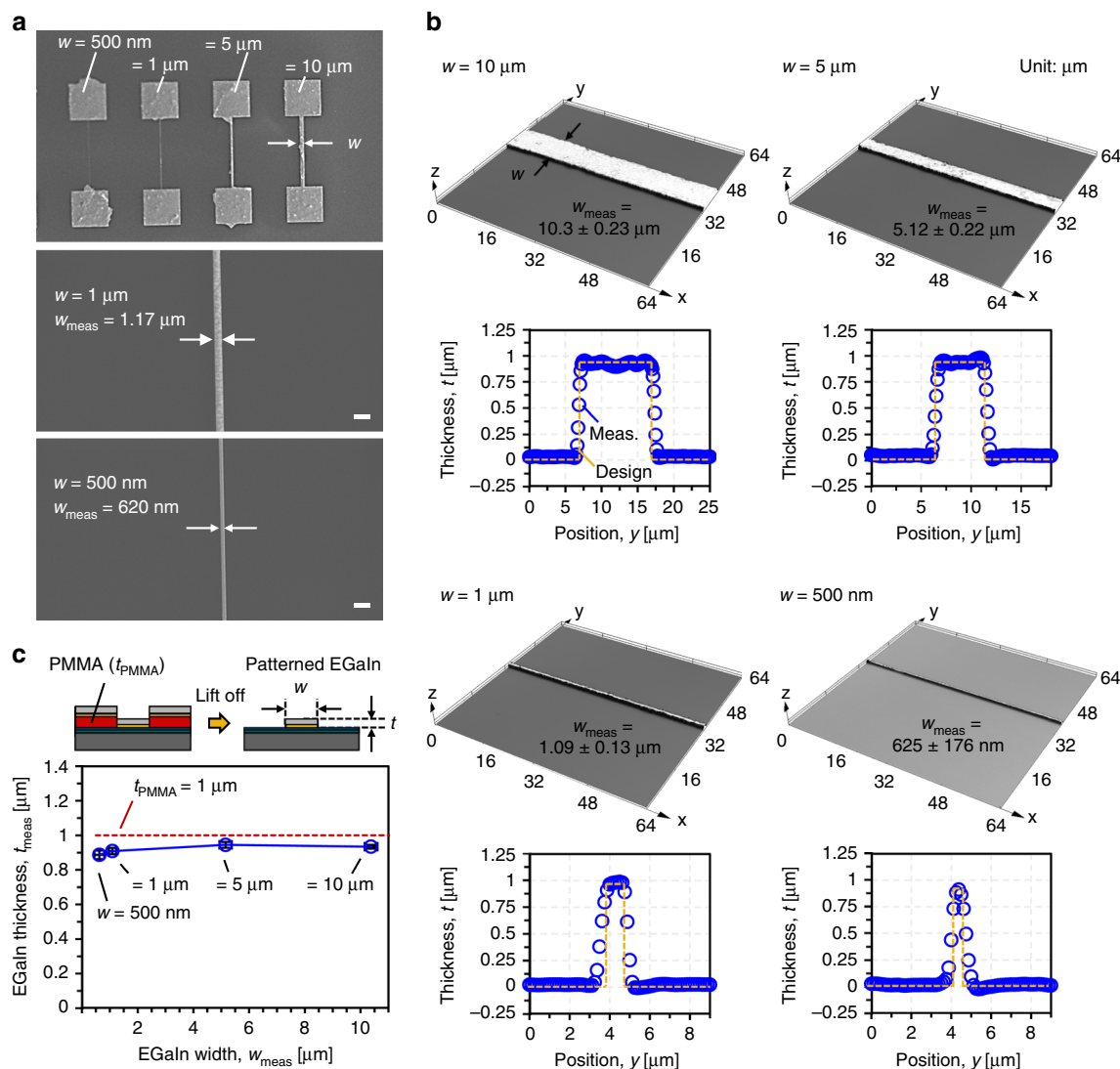
Fig. 2 Patterned EGaIn nano/microstructures. a SEM images of EGaIn lines with widths from 10\ \mu\text{m} to 500\ \text{nm} and close-up of EGaIn lines with 1\ \mu\text{m} and 500\ \text{nm} width. Scale bars indicate 2\ \mu\text{m} . b 3D images and cross-sections of EGaIn lines with width of 10\ \mu\text{m} , 5\ \mu\text{m} , 1\ \mu\text{m} , and 500\ \text{nm} . The blue symbols represent the measured profile, while the dashed yellow line indicates the designed cross-section. c Measured thickness of fabricated EGaIn lines as a function of line width. The x- and y-error bars represent the standard deviation. The thickness of the PMMA film ( 1\ \mu\text{m} ) is shown as dashed red line for reference.
