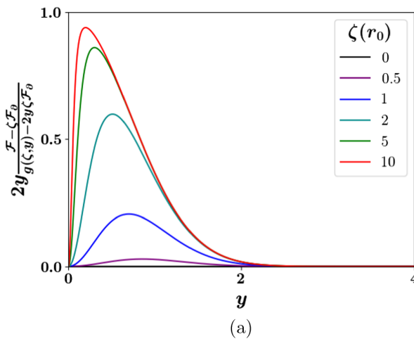
FIG. 4. Analysis of the functions in r' = \frac{r}{r_0} (1 - \frac{2y\zeta\mathcal{F}_\partial}{g(\zeta, y)}) (1 + 2D_{02}y \frac{\mathcal{F} - \zeta\mathcal{F}_\partial}{g(\zeta, y) - 2y\zeta\mathcal{F}_\partial}) , where y = \sqrt{\frac{r}{r_0}} , for various values of \zeta = \frac{r_0\omega_{02}}{2c} . Notice that y is monotonic increasing in r for a given r_0 . The term \frac{2y\zeta\mathcal{F}_\partial}{g(\zeta, y)} is plotted in (a) and shows that (1 - \frac{2y\zeta\mathcal{F}_\partial}{g(\zeta, y)}) is greater than 0 for y > 0 . The term 2y \frac{\mathcal{F} - \zeta\mathcal{F}_\partial}{g(\zeta, y) - 2y\zeta\mathcal{F}_\partial} is plotted in (b). Notice that the max of this second function decreases as \zeta is increased.
