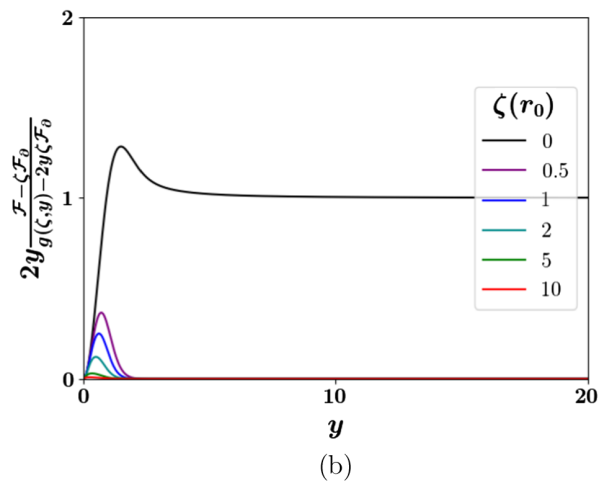
FIG. 4. Analysis of the functions in r' = \frac{r}{r_0} (1 - \frac{2y\zeta\mathcal{F}_\partial}{g(\zeta, y)}) (1 + 2D_{02}y \frac{\mathcal{F} - \zeta\mathcal{F}_\partial}{g(\zeta, y) - 2y\zeta\mathcal{F}_\partial}) , where y = \sqrt{\frac{r}{r_0}} , for various values of \zeta = \frac{r_0\omega_{02}}{2c} . Notice that y is monotonic increasing in r for a given r_0 . The term \frac{2y\zeta\mathcal{F}_\partial}{g(\zeta, y)} is plotted in (a) and shows that (1 - \frac{2y\zeta\mathcal{F}_\partial}{g(\zeta, y)}) is greater than 0 for y > 0 . The term 2y \frac{\mathcal{F} - \zeta\mathcal{F}_\partial}{g(\zeta, y) - 2y\zeta\mathcal{F}_\partial} is plotted in (b). Notice that the max of this second function decreases as \zeta is increased.
