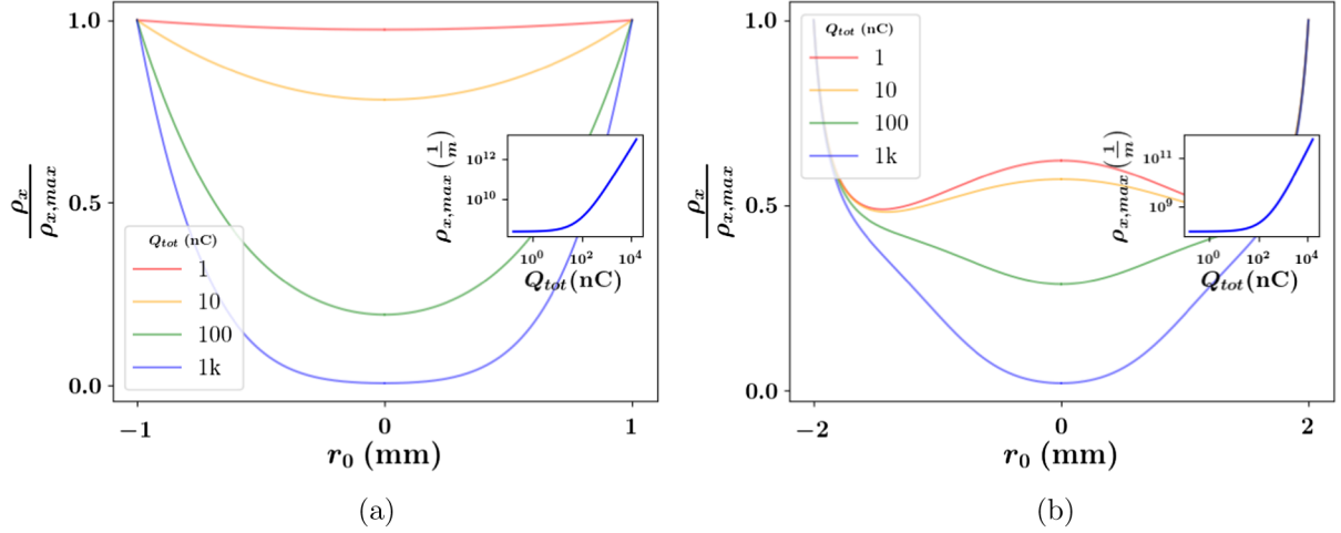
FIG. 9. The shape of \frac{\rho_x}{\rho_{x,max}} for various values of Q_{tot,3} in (a) an initially uniform distribution with radius of 1 mm and (b) an initially Gaussian distribution with standard deviation of 1 mm as a function of the initial radial coordinate. This, as well as the inset figure describing the growth of the maximum value of \rho_{x3} , show the onset of the relativistic regime corresponding to roughly 24 \frac{c}{m} . The main graph also shows that the peaks sharpen as the density increases. For the Gaussian case, this distribution diverges near r_0 = 2 . This divergence is an indication that the laminar fluid assumption is being violated, and therefore the nonuniform asymptote for \rho_{x3} should be taken as a gross approximation; nonetheless, the expression derived in the text do capture the shape of freely-expanding relativistic Gaussian distribution in the simulation presented in Fig. 7.
