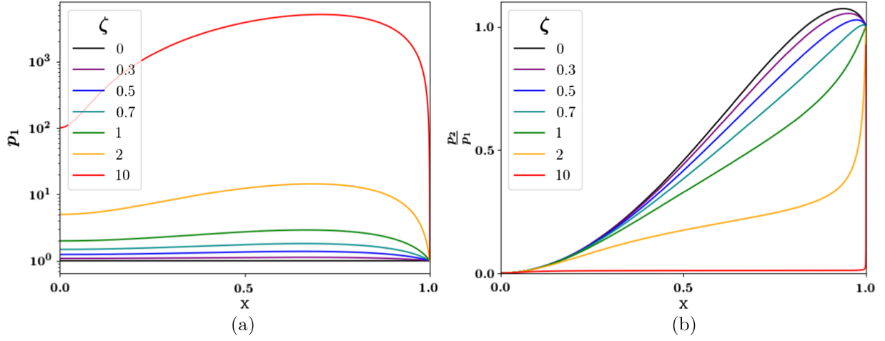
FIG. 6. Analysis of the functions in r' = \frac{r}{r_0} \frac{p_1(x)}{g_1(1)g_2(x)} (1 + \frac{3}{2} D_{03} \frac{p_2(x)}{p_1(x)}) , where p_1 , p_2 , g_1 , and g_2 are defined in the text. Notice that x^2 = 1 - \frac{r_0}{r} has a range [0, 1] with x = 0 occurring at t = 0 and x = 1 occurring at t = \infty . The term p_1(x) is plotted in (a) and shows that p_1(x) is greater than 0 for x > 0 . The term \frac{p_2}{p_1} is plotted in (b). Notice that the value of this second function for a specific x in (0,1) decreases as \zeta is increased.
