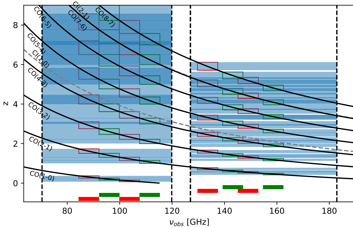
Fig. 1. Spectral coverage of the ^{12}\text{CO} (solid black) and [\text{CI}] (dashed gray) emission lines as a function of redshift in the 3 and 2 mm atmospheric windows in the frequency ranges 84–115 GHz and 130–163 GHz. The bottom colored boxes show the LSB and USB frequency settings (red and green, respectively) (see Table 2). The 2 mm frequency windows were selected to optimally cover the range of spectroscopic redshifts predicted by the 3 mm observations. The dark blue zones identify the redshift ranges where at least two emission lines are detected at 3 or 2 mm with the current settings, while the light blue zones indicate the redshift ranges where only one line is present. This wide frequency range enables the detection of at least one emission line in each band, except for a few small redshifts gaps (see Sect. 2 for details).
