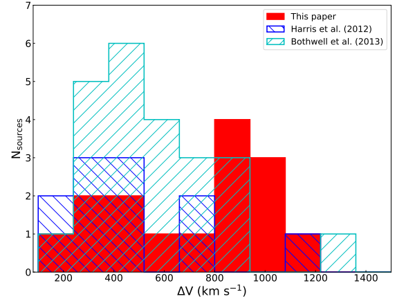
Fig. 10. Distribution of the full width at half maximum (FWHM) for the bright Herschel galaxies detected in ^{12}\text{CO} described in this paper (solid red histogram) compared to the FWHM of high- z galaxies reported in Bothwell et al. (2013) (cyan right-hatched) and Harris et al. (2012) (blue left-hatched).
