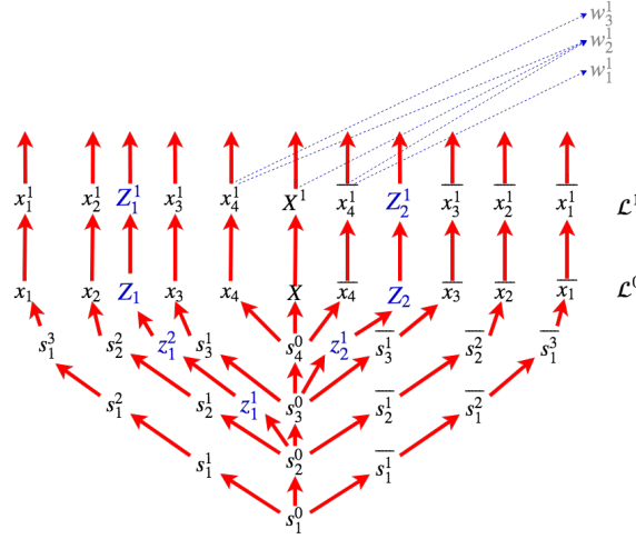
■ Figure 4 Vertex Z_1 and Z_2 could be for clauses (x_1, x_2, x_3) , (x_2, \overline{x_3}, x_4) . Each “betweenness” constraint adds a layer. (x_4, X, \overline{x_4}) constraint shown.
