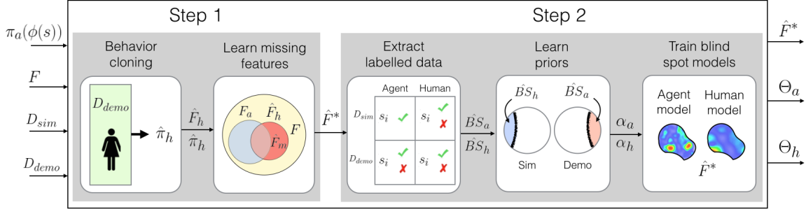
Figure 2: Pipeline of approach. The first step involves learning missing features that the agent learned to ignore in simulation. The second step is learning agent and human blind spot models in the real world, which involves extracting labeled data, learning priors of blind spots, and finally training the supervised learning models.
