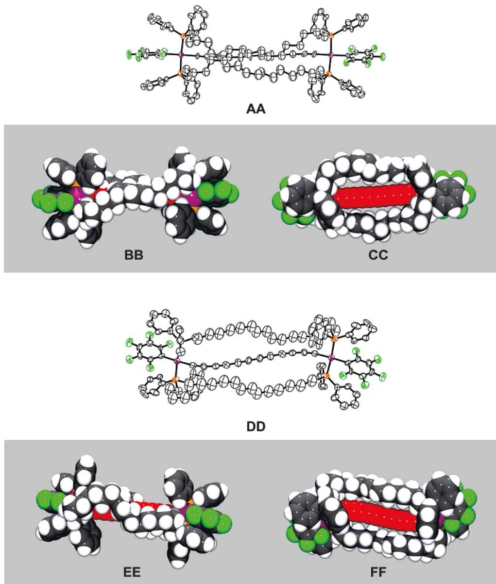
Figure 6. Structures of the two independent Pt(C≡C) 12 Pt complexes in crystalline 11 (CH 2 Cl 2 ) 0.67 with solvate molecules omitted: AA , thermal ellipsoid plot (50% probability level) of the double-helical complex with hydrogen atoms omitted; BB , CC , views parallel and perpendicular to the planes of the C 6 F 5 ligands with atoms at van der Waals radii; DD , EE , FF , analogous views of the nonhelical complex.
