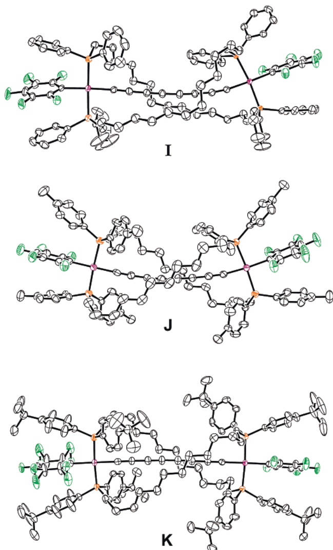
Figure 1. Thermal ellipsoid plots (50% probability level) of the double-helical \text{Pt}(\text{C}\equiv\text{C})_4\text{Pt} complexes with hydrogen atoms and solvate molecules omitted: I , 3 (toluene) 1.5 ; J , 4 ; K , 5 (toluene) 5.5 .
