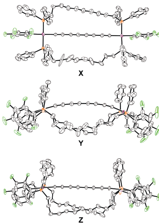
Figure 5. Thermal ellipsoid plots (50% probability level) of other nonhelical \text{Pt}(\text{C}\equiv\text{C})_4\text{Pt} complexes with hydrogen atoms and solvate molecules omitted: X , 7 (toluene) 4 (dominant conformation); Y , 7 ( \text{CHCl}_3 ) 2 ; Z , 9 ( \text{CH}_2\text{Cl}_2 ) 2.5 (dominant conformation).
