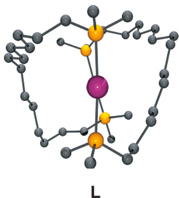
Figure 2. View of 3 (toluene) 1.5 along the platinum–platinum axis with non- ipso aryl carbon atoms, hydrogen atoms, and solvate molecules omitted.
