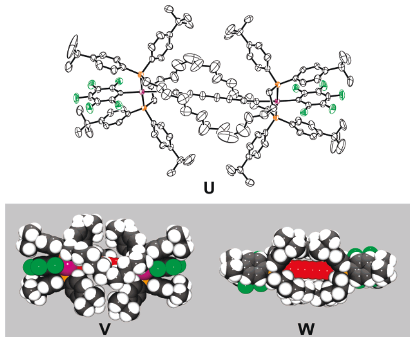
Figure 4. Structure of the nonhelical \text{Pt}(\text{C}\equiv\text{C})_4\text{Pt} complex 5 (toluene) 2 with solvate molecules omitted: U , thermal ellipsoid plot (50% probability level) with hydrogen atoms omitted; V , W , views parallel and perpendicular to the planes of the \text{C}_6\text{F}_5 ligands with atoms at van der Waals radii.
