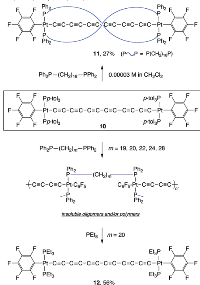
Scheme 5. Reactions of the \text{Pt}(\text{C}\equiv\text{C})_6\text{Pt} Complex 10 with Bis( \alpha , -diphenylphosphino)alkanes
