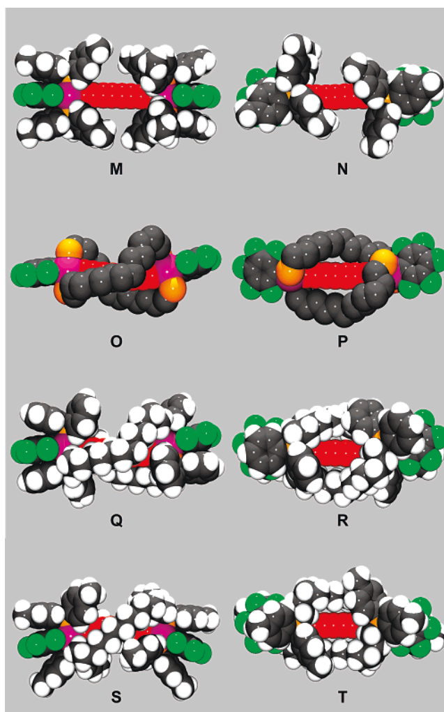
Figure 3. Space filling representations of selected \text{Pt}(\text{C}\equiv\text{C})_4\text{Pt} complexes: M , N , views of 2 (toluene) parallel and perpendicular to the planes of the \text{C}_6\text{F}_5 ligands; O , P , analogous views of 3 (toluene) 1.5 with phenyl rings, hydrogen atoms, and solvate molecules omitted; Q , R , analogous views of 3 (toluene) 1.5 but with phenyl rings and hydrogen atoms; S , T , analogous views of 4 .
