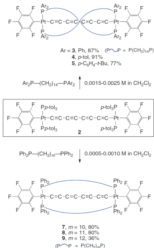
Scheme 4. Reactions of the Pt(C≡C) 4 Pt Complex 2 with Bis(α, -diarylphosphino)alkanes
