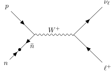
Fig. 3. Feynman diagram for np \rightarrow \ell^+ \nu_\ell , where \ell = e, \mu, \tau .
