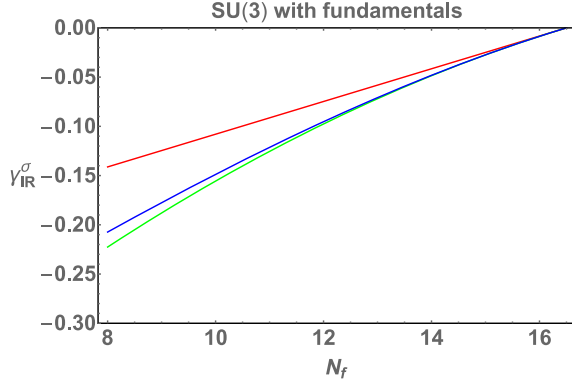
FIG. 4. Plot of the anomalous dimension \gamma_{IR,F}^{(\sigma)} of the operator \bar{\psi}\sigma_{\lambda\mu_1}\psi at the IRFP for G = \text{SU}(3) , and N_f fermions in the fundamental representation, calculated to order O(\Delta_f^p) , where p = 1, 2, 3 . Denoting the calculation to order O(\Delta_f^p) as \gamma_{IR,F,\Delta_f^p}^{(\sigma)} , the colors refer to \gamma_{IR,F,\Delta_f^1}^{(\sigma)} (red), \gamma_{IR,F,\Delta_f^2}^{(\sigma)} (green), and \gamma_{IR,F,\Delta_f^3}^{(\sigma)} (blue).
