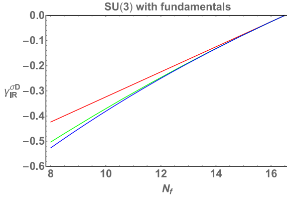
FIG. 5. Plot of the anomalous dimension \gamma_{IR,F}^{(\sigma D)} of the operator \bar{\psi}\sigma_{\lambda\mu_1}D_{\mu_2}\psi at the IRFP for G = \text{SU}(3) , and N_f fermions in the fundamental representation, calculated to order O(\Delta_f^p) , where p = 1, 2, 3 . Denoting the calculation to order O(\Delta_f^p) as \gamma_{IR,F,\Delta_f^p}^{(\sigma D)} , from top to bottom, the colors refer to \gamma_{IR,F,\Delta_f^1}^{(\sigma D)} (red), \gamma_{IR,F,\Delta_f^2}^{(\sigma D)} (green), and \gamma_{IR,F,\Delta_f^3}^{(\sigma D)} (blue).
