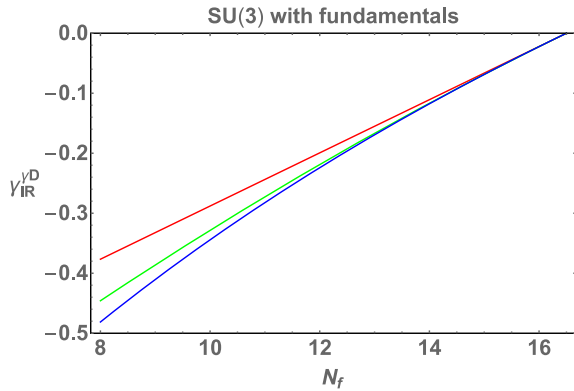
FIG. 1. Plot of the anomalous dimension \gamma_{\text{IR},F}^{(D)} of the operator \bar{\psi}\gamma_{\mu_1}D_{\mu_2}\psi at the IRFP for the theory with G = \text{SU}(3) , and N_f fermions in the fundamental representation, calculated to order O(\Delta_f^p) , where p = 1, 2, 3 . Denoting the anomalous dimension calculated to order O(\Delta_f^p) as \gamma_{\text{IR},F,\Delta_f^p}^{(D)} , the curves, from top to bottom, refer to \gamma_{\text{IR},F,\Delta_f}^{(D)} (red), \gamma_{\text{IR},F,\Delta_f^2}^{(D)} (green), and \gamma_{\text{IR},F,\Delta_f^3}^{(D)} (blue).
