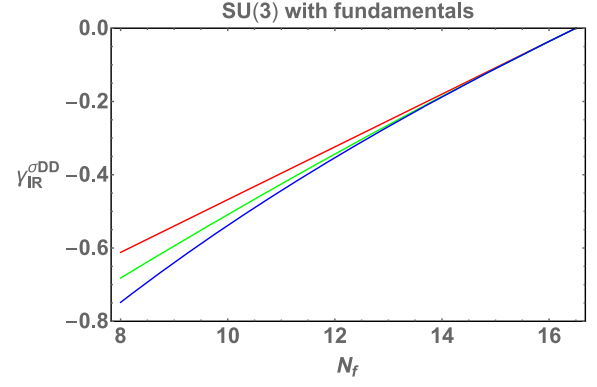
FIG. 6. Plot of the anomalous dimension \gamma_{IR,F}^{(\sigma DD)} of the operator \bar{\psi}\sigma_{\lambda\mu_1}D_{\mu_2}D_{\mu_3}\psi at the IRFP for G = \text{SU}(3) , and N_f fermions in the fundamental representation, calculated to order O(\Delta_f^p) , where p = 1, 2, 3 . Denoting the calculation to order O(\Delta_f^p) as \gamma_{IR,F,\Delta_f^p}^{(\sigma DD)} , from top to bottom, the colors refer to \gamma_{IR,F,\Delta_f^1}^{(\sigma DD)} (red), \gamma_{IR,F,\Delta_f^2}^{(\sigma DD)} (green), and \gamma_{IR,F,\Delta_f^3}^{(\sigma DD)} (blue).
