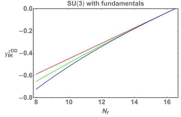
FIG. 2. Plot of the anomalous dimension \gamma_{\text{IR},F}^{(DD)} of the operator \bar{\psi}\gamma_{\mu_1}D_{\mu_2}D_{\mu_3}\psi at the IRFP for G = \text{SU}(3) , and N_f fermions in the fundamental representation, calculated to order O(\Delta_f^p) , where p = 1, 2, 3 . Denoting the anomalous dimension calculated to order O(\Delta_f^p) as \gamma_{\text{IR},F,\Delta_f^p}^{(DD)} , the curves, from top to bottom, refer to \gamma_{\text{IR},F,\Delta_f}^{(DD)} (red), \gamma_{\text{IR},F,\Delta_f^2}^{(DD)} (green), and \gamma_{\text{IR},F,\Delta_f^3}^{(DD)} (blue).
