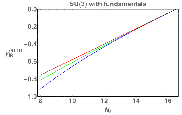
FIG. 7. Plot of the anomalous dimension \gamma_{IR,F}^{(\sigma DDD)} of the operator \bar{\psi}\sigma_{\lambda\mu_1}D_{\mu_2}D_{\mu_3}D_{\mu_4}\psi at the IRFP for G = \text{SU}(3) , and N_f fermions in the fundamental representation, calculated to order O(\Delta_f^p) , where p = 1, 2, 3 . Denoting the calculation to order O(\Delta_f^p) as \gamma_{IR,F,\Delta_f^p}^{(\sigma DDD)} , from top to bottom, the colors refer to \gamma_{IR,F,\Delta_f^1}^{(\sigma DDD)} (red), \gamma_{IR,F,\Delta_f^2}^{(\sigma DDD)} (green), and \gamma_{IR,F,\Delta_f^3}^{(\sigma DDD)} (blue).
