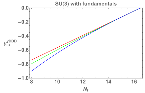
FIG. 3. Plot of the anomalous dimension \gamma_{\text{IR},F}^{(DDD)} of the operator \bar{\psi}\gamma_{\mu_1}D_{\mu_2}D_{\mu_3}D_{\mu_4}\psi at the IRFP for G = \text{SU}(3) , and N_f fermions in the fundamental representation, calculated to order O(\Delta_f^p) , where p = 1, 2, 3 . Denoting the calculation to order O(\Delta_f^p) as \gamma_{\text{IR},F,\Delta_f^p}^{(DDD)} , from top to bottom, the colors refer to \gamma_{\text{IR},F,\Delta_f}^{(DDD)} (red), \gamma_{\text{IR},F,\Delta_f^2}^{(DDD)} (green), and \gamma_{\text{IR},F,\Delta_f^3}^{(DDD)} (blue).
