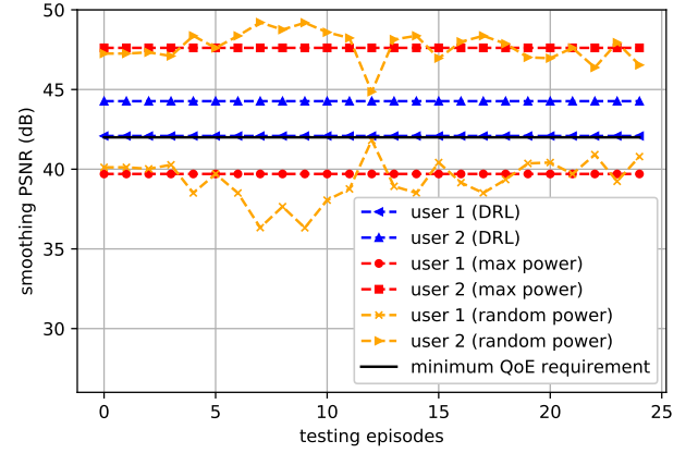
FIGURE 8. Users' QoE versus the number of testing episodes ( N = 2 ).
