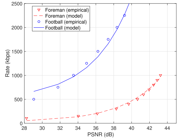
FIGURE 3. Rate-distortion curve for the two video sequences.
