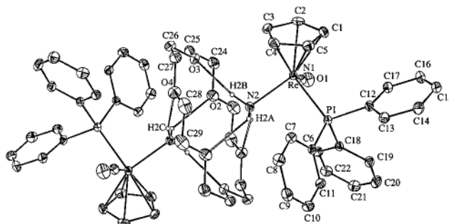
Figure 2. Structure of the dication of 2^{2+}2\text{PF}_6^- \cdot \text{OEt}_2 .
