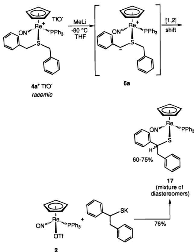
Scheme 9. Generation and Independent Synthesis of a [1,2]-Rearrangement Product
