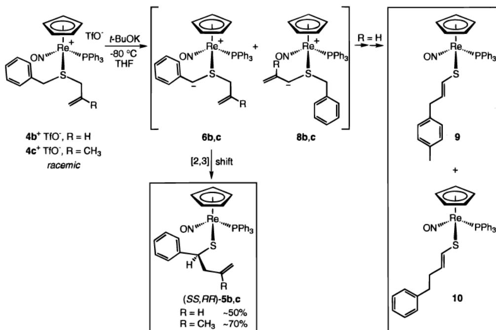
Scheme 6. Reactions of Allyl \beta -Keto Sulfide Complexes 4d-f + X -
