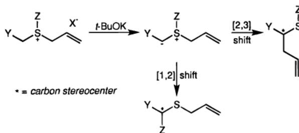
Scheme 1. Generation and Rearrangements of Allyl-Substituted Sulfur Ylides
