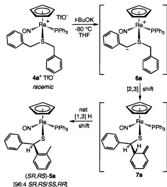
Scheme 4. Reaction of Dibenzyl Sulfide Complex 4a^+\text{TfO}^-
