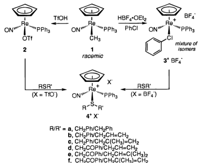
Scheme 3. Syntheses of New Sulfide Complexes
