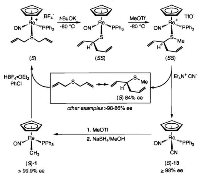
Scheme 3. Syntheses of New Sulfide Complexes
