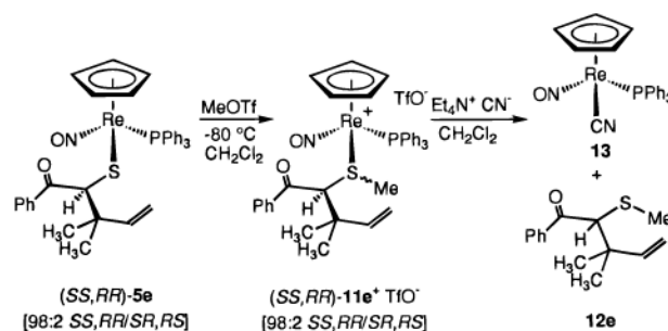
Scheme 7. Detachment of Thiolate Ligands
