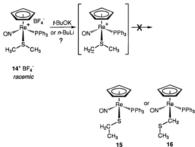
Scheme 8. Attempted Reactions of Dimethyl Sulfide Complex 14^+BF_4^-
