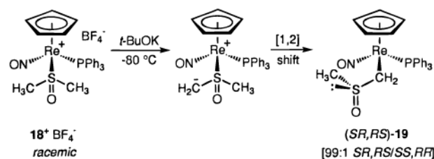
Scheme 10. Reaction of DMSO Complex 18 + BF 4 −
