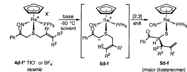
Scheme 6. Reactions of Allyl \beta -Keto Sulfide Complexes 4d-f + X -
