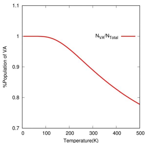
Fig. 8 Ratio of the Boltzmann population of VA ( N_{\text{VA}} ) relative to the total population ( N_{\text{Total}} ) as a function of temperature.
