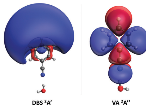
Fig. 6 Dyson orbitals for the two lowest electronic states of the \text{C}_6\text{H}_5\text{CN} \cdot \text{H}_2\text{O} complex, ^2\text{A}' and ^2\text{A}'' , computed at the respective optimized geometries. Isovalue 0.007.
