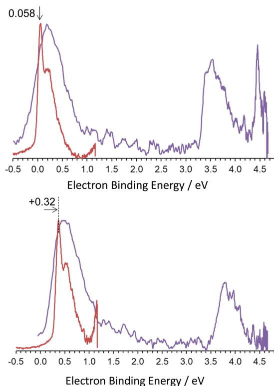
Fig. 1 Photoelectron spectra of \text{C}_6\text{H}_5\text{CN}^- (top) and \text{C}_6\text{H}_5\text{CN}^-\cdot\text{H}_2\text{O} (bottom) obtained with two different photon energies. Red and blue lines correspond to the spectra obtained with 1.165 eV and 4.661 eV photons, respectively. Reproduced with permission from ref. 24.
