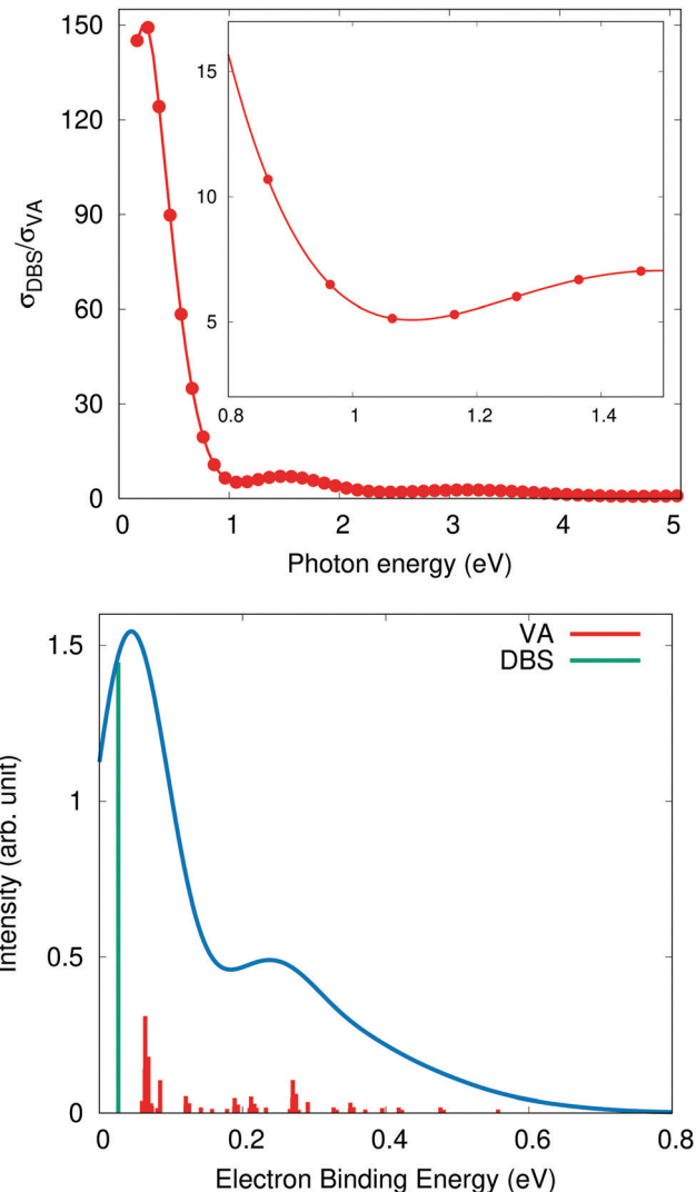
Fig. 11 Top: Ratio of the cross sections (DBS versus VA) for electron detachment from the benzonitrile anion. Bottom: Convolution of the Franck–Condon factors using eqn (15) with Gaussian (width = 0.05 eV) and assuming equal populations of the DBS and VA.
