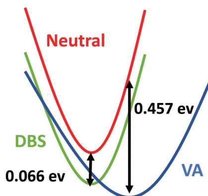
Fig. 7 Schematic representation of the neutral, valence anions, and dipole-bound states of the benzonitrile–water complex.
