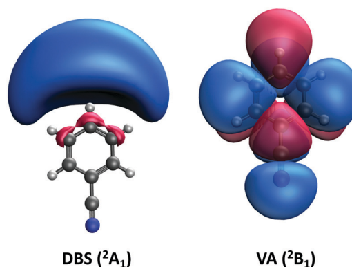
Fig. 3 Dyson orbitals for the two lowest electronic states of the benzonitrile anion, ^2\text{A}_1 and ^2\text{B}_1 , computed at the respective optimized geometries. Isovalue 0.007.
