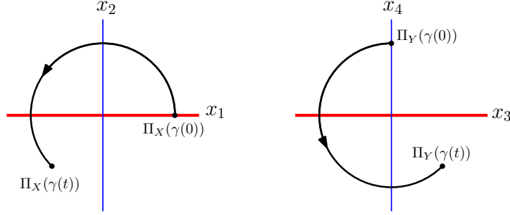
Figure 1: Subgradient curve \gamma(\cdot) generated by f is depicted in the figure with an arrow; the set of critical points of f is the product of the x_1 and x_3 axes. The picture on the left shows the projection of \gamma onto the coordinate X = (x_1, x_2) , while the picture on the right shows the projection of \gamma onto the coordinates Y = (x_3, x_4) .
