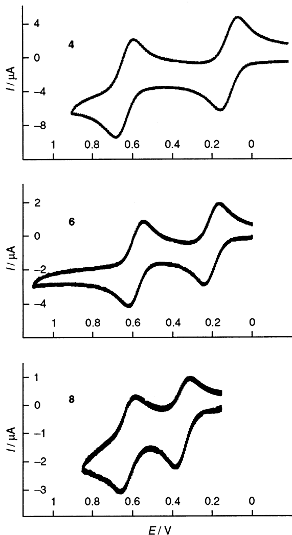
Fig. 2 Cyclic voltammograms of 4 , 6 and 8 ( 7\text{--}8 \times 10^{-5}\text{ mol dm}^{-3} in 0.1\text{ mol dm}^{-3}\text{ Bu}_4\text{N}^+\text{BF}_4^-\text{CH}_2\text{Cl}_2 at ambient temperature; Pt working and counter electrodes, ferrocene standard, potential vs. Ag wire pseudoreference; scan rate 100\text{ mV s}^{-1} )
