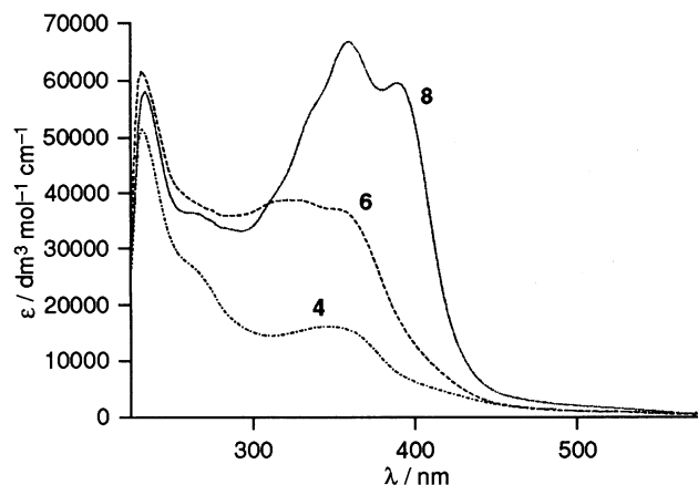
Fig. 1 UV-VIS spectra of 4 , 6 and 8 ( 1.6\text{--}3.3 \times 10^{-5}\text{ mol dm}^{-3} in \text{CH}_2\text{Cl}_2 at ambient temperature)
