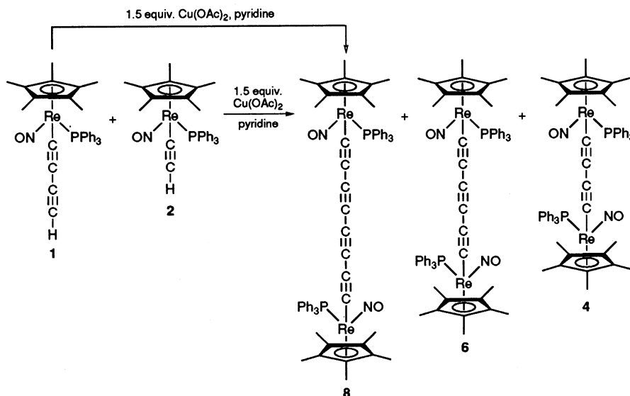
Scheme 1 Coupling and cross-coupling of 1,3-butadiynyl complex 1
