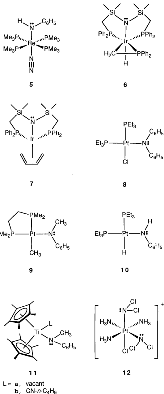
Figure 3. Some relevant structurally characterized transition-metal amido complexes
