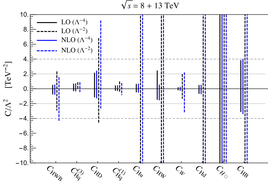
FIG. 6. The 95% confidence interval fits to individual EFT coefficients using W^+W^- + W^\pm Z + ZH + W^\pm H data and profiling over all other coefficients. Fits quadratic in 1/\Lambda^2 (linear) LO and NLO QCD are shown as solid (dashed) black and blue lines, respectively.
