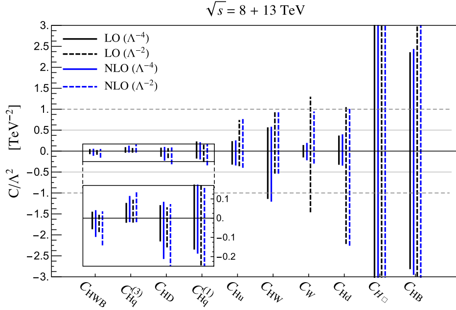
FIG. 5. The 95% confidence interval fits to individual EFT coefficients using W^+W^- + W^\pm Z + ZH + W^\pm H data. All other SMEFT coefficients are projected to zero. Fits quadratic in 1/\Lambda^2 (linear) LO and NLO QCD are shown as solid (dashed) black and blue lines, respectively.
