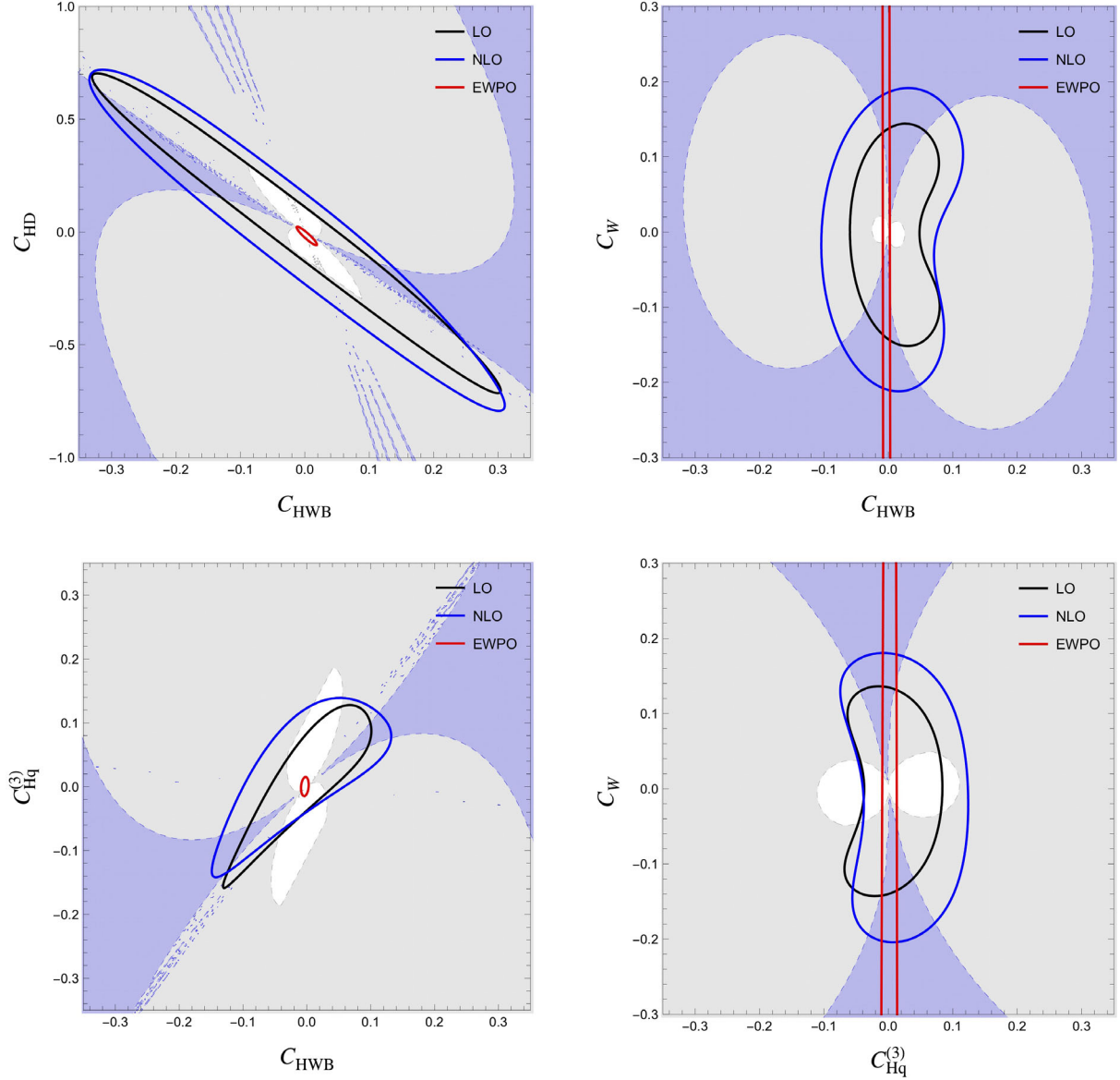
FIG. 7. The 95% confidence region in the C_{HWB} - C_{HD} (top left), C_{HWB} - C_W (top right), C_{HWB} - C_{Hq}^{(3)} (bottom left), and C_{Hq}^{(3)} - C_W (bottom right) planes with all other EFT coefficients projected to zero and \Lambda fixed to 1 TeV. Quadratic fits to W^+W^- + W^\pm Z + ZH + W^\pm H distributions are shown in black (blue) for LO (NLO) QCD in SMEFT, while the quadratic fit to NLO electroweak precision observables is shown in red. The grey (blue) region indicates the coefficients no longer correspond to a weakly coupled theory that is \Delta\sigma_{\Lambda^4} > \Delta\sigma_{\Lambda^2}(4\pi\Delta\sigma_{\Lambda^2}) .
