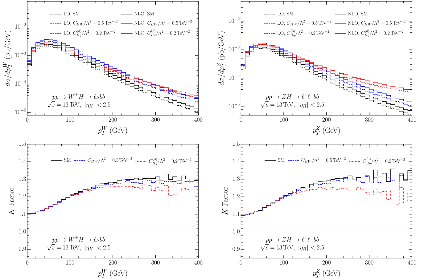
FIG. 1. Top: Differential distributions for W^\pm H (left) and ZH (right) production at LO (dashed lines) and NLO (solid lines) in bins of p_T^V . We plot the results for the SM (black lines), C_{HW}/\Lambda^2 = 0.5 \text{ TeV}^{-2} (blue lines), and C_{Hq}^{(3)}/\Lambda^2 = 0.2 \text{ TeV}^{-2} (red lines). Bottom: The associated K factors for the same distributions at the same three points, also in bins of p_T^V . The figures are computed to \mathcal{O}(1/\Lambda^4) .
