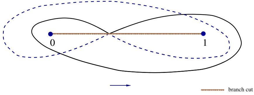
Figure 2. The Pochhammer contour \gamma_P .
