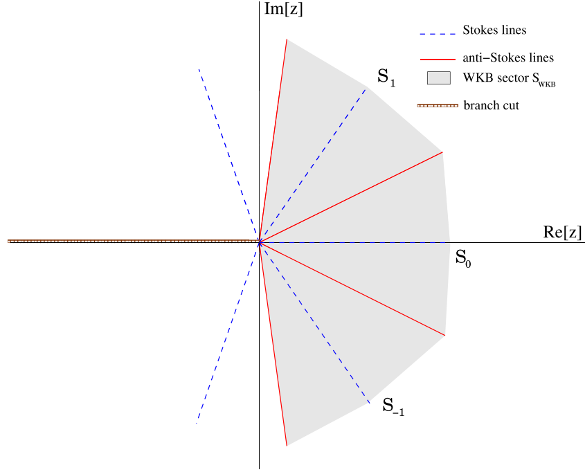
Figure 1. Stokes, WKB sectors and convention for the branch cut when 2M \notin \mathbb{Z}_{\geq} .
