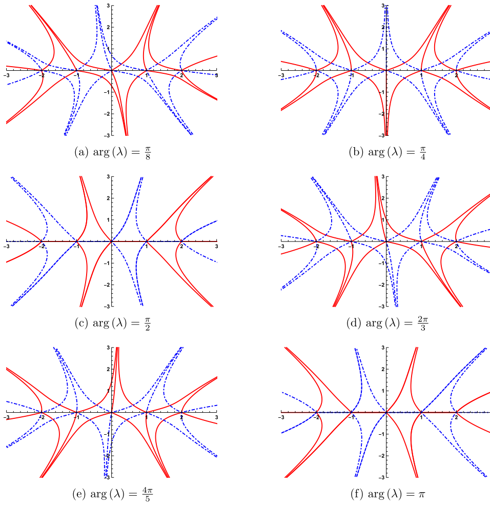
Figure 8. Plots of Stokes and anti-Stokes lines for the polynomial function P(z) = z(z^2 - 1)(z^2 - 4) and various phases of the spectral parameter \lambda . One sees that a counter-clockwise rotation of \lambda corresponds to a clockwise rotation of the sectors. For \arg(\lambda) = \pi , the picture looks the same as figure 6, but the sectors have been exchanged in a clockwise fashion.
