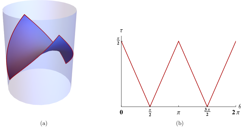
Figure 4. Minimal surface for the case P = \bar{P} = 1 , \alpha = 1 and \varphi = 0 in \text{AdS}_3 and its Wilson loop. (a) is a representation with \tanh(\rho) as a radius, \tau as a vertical direction and \theta as an angle where (\rho, \tau, \theta) are \text{AdS}_3 global coordinates (114). The shaded cylinder is the conformal boundary and the red line is the Wilson loop. (b) is a plot of the Wilson loop on the plane (\theta, \tau) corresponding to the boundary \tanh \rho = 1 .
