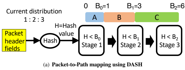
Figure 5: DASH data structure
