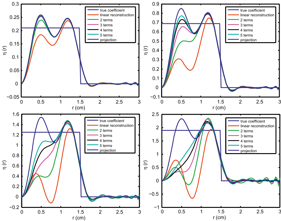
Figure 12.1: Reconstructions of inhomogeneities with R_1 = 1.5 cm and R = 3 cm. The contrast ranges from: top left \eta_0 = 1.1 , top right \eta_0 = 1.3 , bottom left \eta_0 = 1.5 and bottom right \eta_0 = 1.7 .
