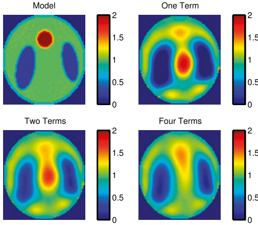
Figure 12.2: Reconstruction of the conductivity with \sigma_{\text{lungs}} = 0.2 and \sigma_{\text{heart}} = 2 .
