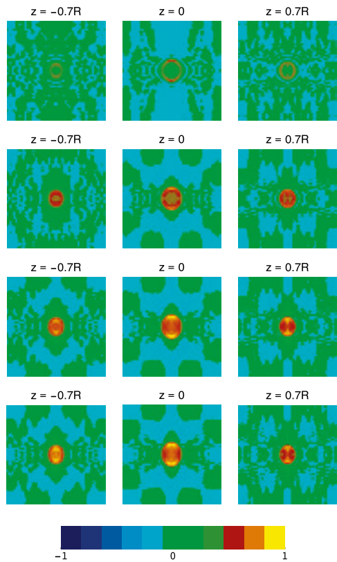
Figure 12.4: Tomographic images of the reconstructed susceptibility.
