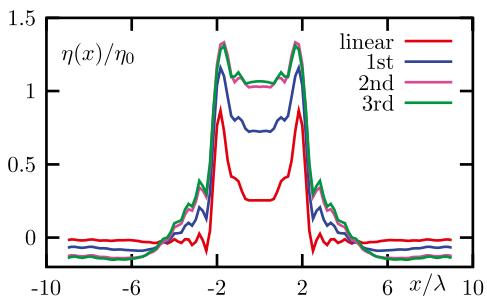
Figure 12.5: One-dimensional profiles of the reconstructed susceptibility.
