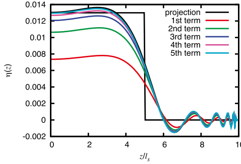
Figure 12.3: Reconstruction of the attenuation coefficient.
