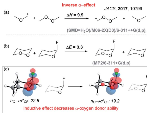
Scheme 3 The magnitude of inverse α-effect in carbenium ions (a) and anomeric systems (b). Comparison of NBO n_{\text{O}} \rightarrow \sigma^*_{\text{CF}} interactions (c) (energies are in kcal mol −1 ).
