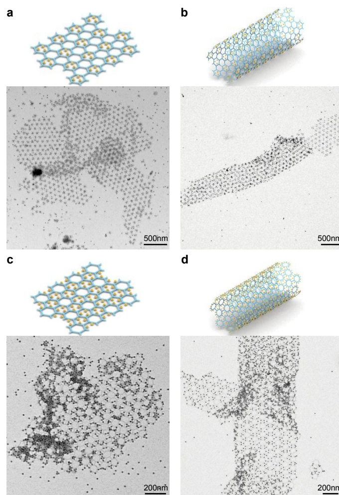
Figure 3. TEM imaging of gold nanoparticle lattices. (a, b) Gold nanoparticle lattices assembled on honeycomb array or tube with type-1 configuration. (c, d) Gold nanoparticle lattices assembled on honeycomb array or tube with type-2 configuration.
